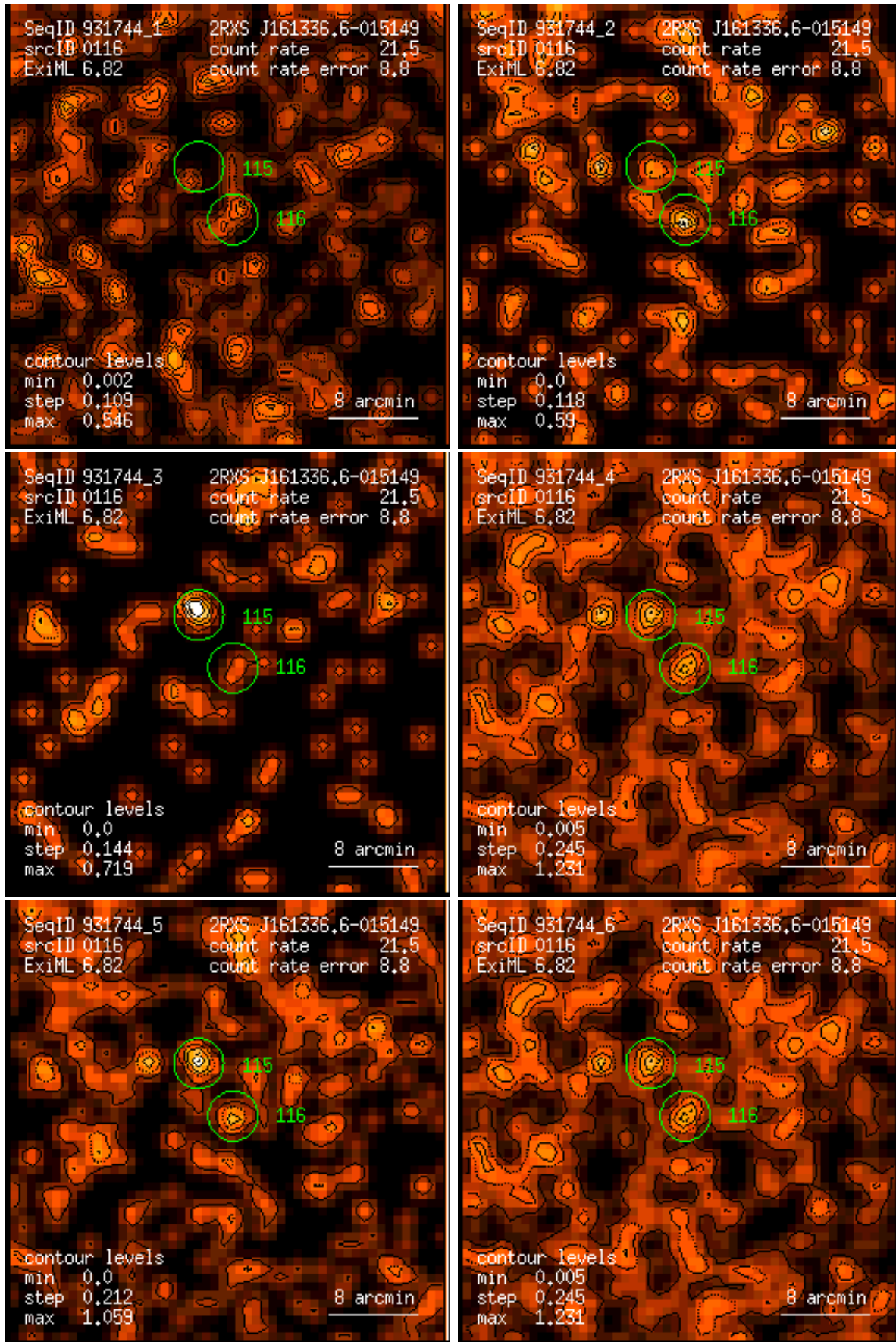
Figure 116: RASS 931744: detection 0116: band rate images, Gaussian filter: (1) PSPC channels 11 – 41, (2) 52 – 90, (3) 91 – 201, (4) 11 – 235, (5) 52 – 201, (6) 11 – 201. Broad band rates in counts/ks. Band rate contour levels in counts/ks/arcmin 2 .
