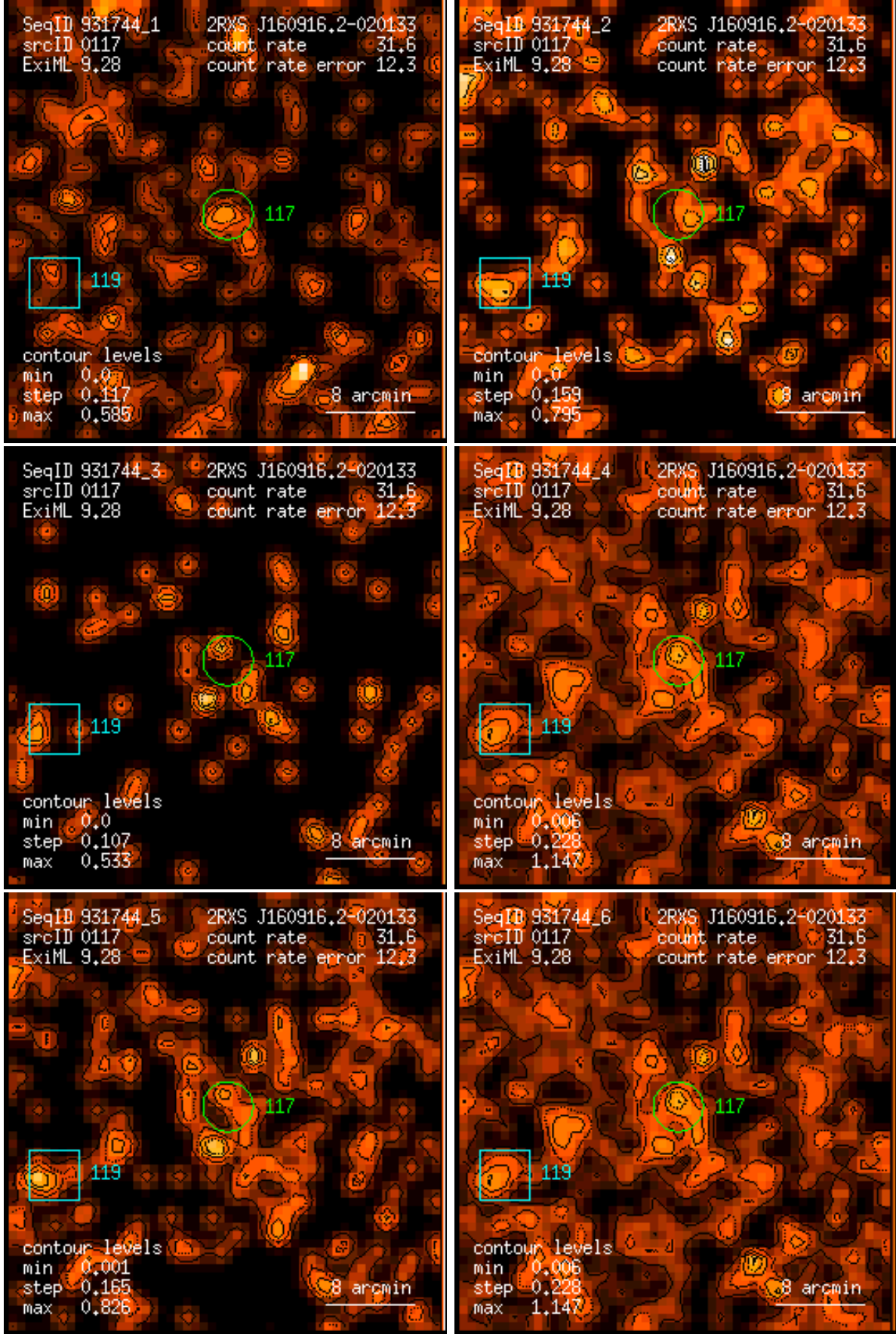
Figure 117: RASS 931744: detection 0117: band rate images, Gaussian filter: (1) PSPC channels 11 – 41, (2) 52 – 90, (3) 91 – 201, (4) 11 – 235, (5) 52 – 201, (6) 11 – 201. Broad band rates in counts/ks. Band rate contour levels in counts/ks/arcmin 2 .
