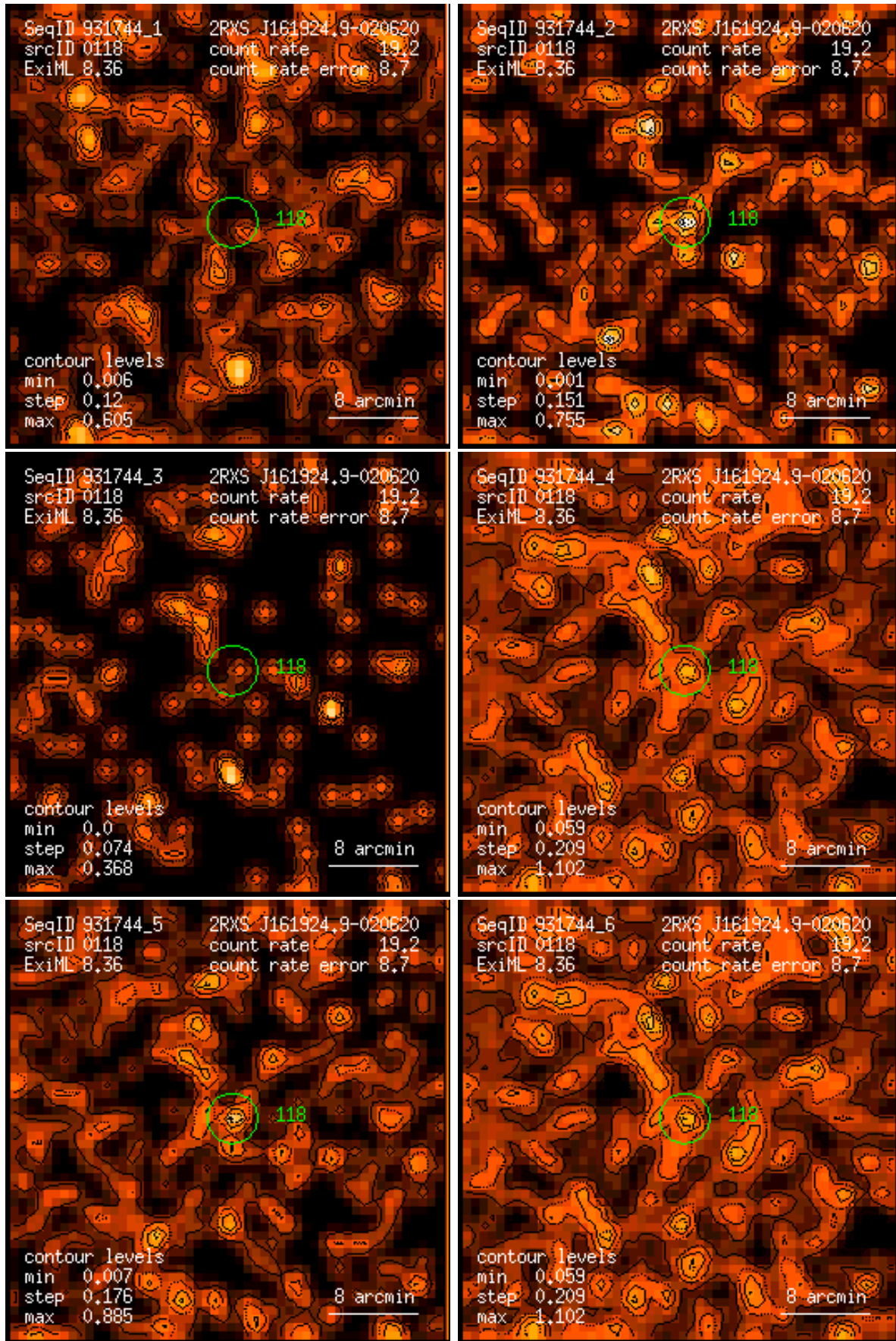
Figure 118: RASS 931744: detection 0118: band rate images, Gaussian filter: (1) PSPC channels 11 – 41, (2) 52 – 90, (3) 91 – 201, (4) 11 – 235, (5) 52 – 201, (6) 11 – 201. Broad band rates in counts/ks. Band rate contour levels in counts/ks/arcmin 2 .
