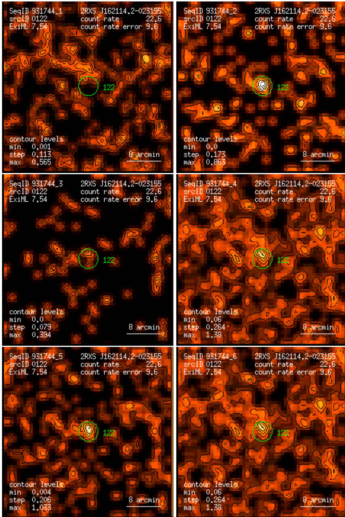
Figure 122: RASS 931744: detection 0122: band rate images, Gaussian filter: (1) PSPC channels 11 – 41, (2) 52 – 90, (3) 91 – 201, (4) 11 – 235, (5) 52 – 201, (6) 11 – 201. Broad band rates in counts/ks. Band rate contour levels in counts/ks/arcmin 2 .
