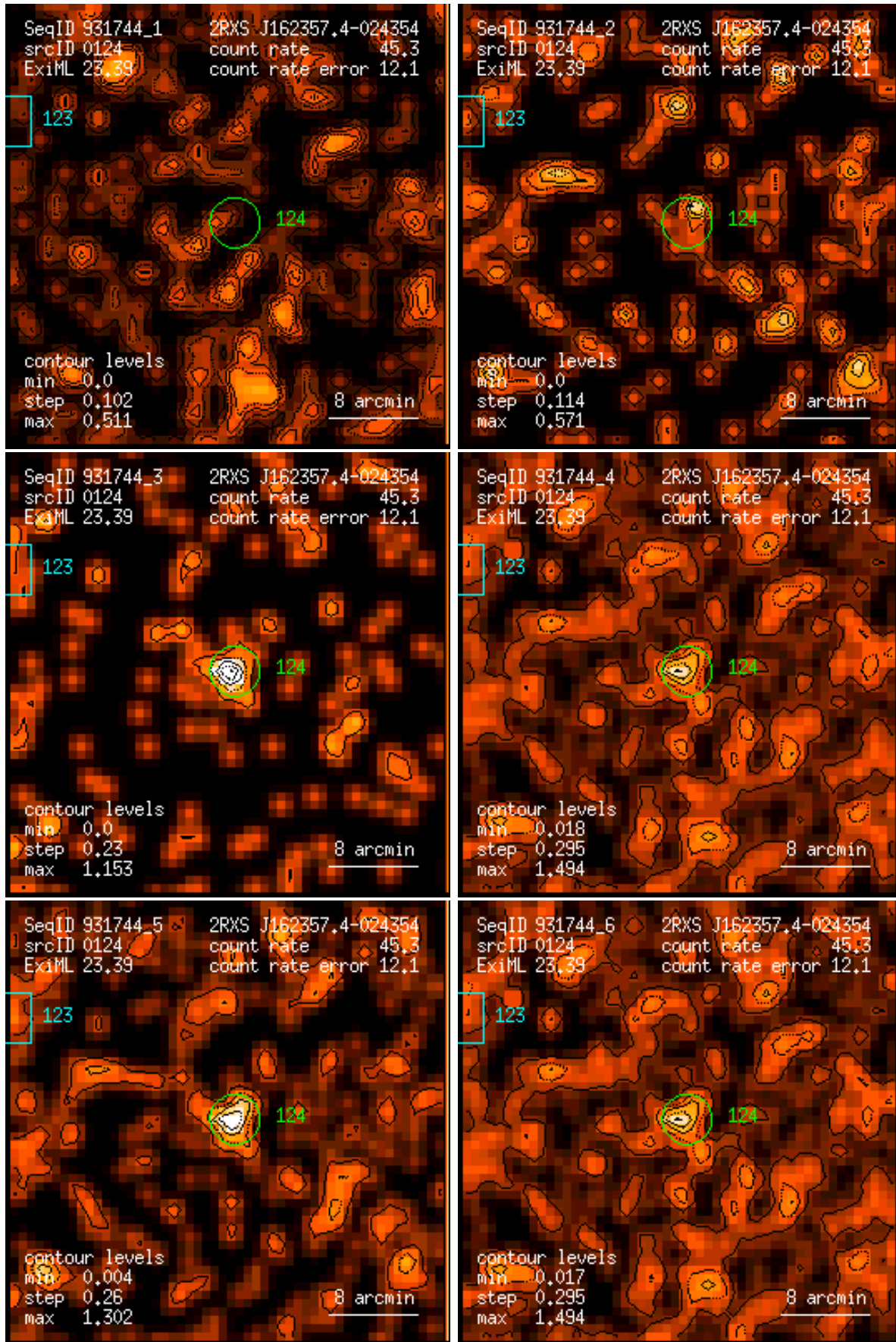
Figure 124: RASS 931744: detection 0124: band rate images, Gaussian filter: (1) PSPC channels 11 – 41, (2) 52 – 90, (3) 91 – 201, (4) 11 – 235, (5) 52 – 201, (6) 11 – 201. Broad band rates in counts/ks. Band rate contour levels in counts/ks/arcmin 2 .
