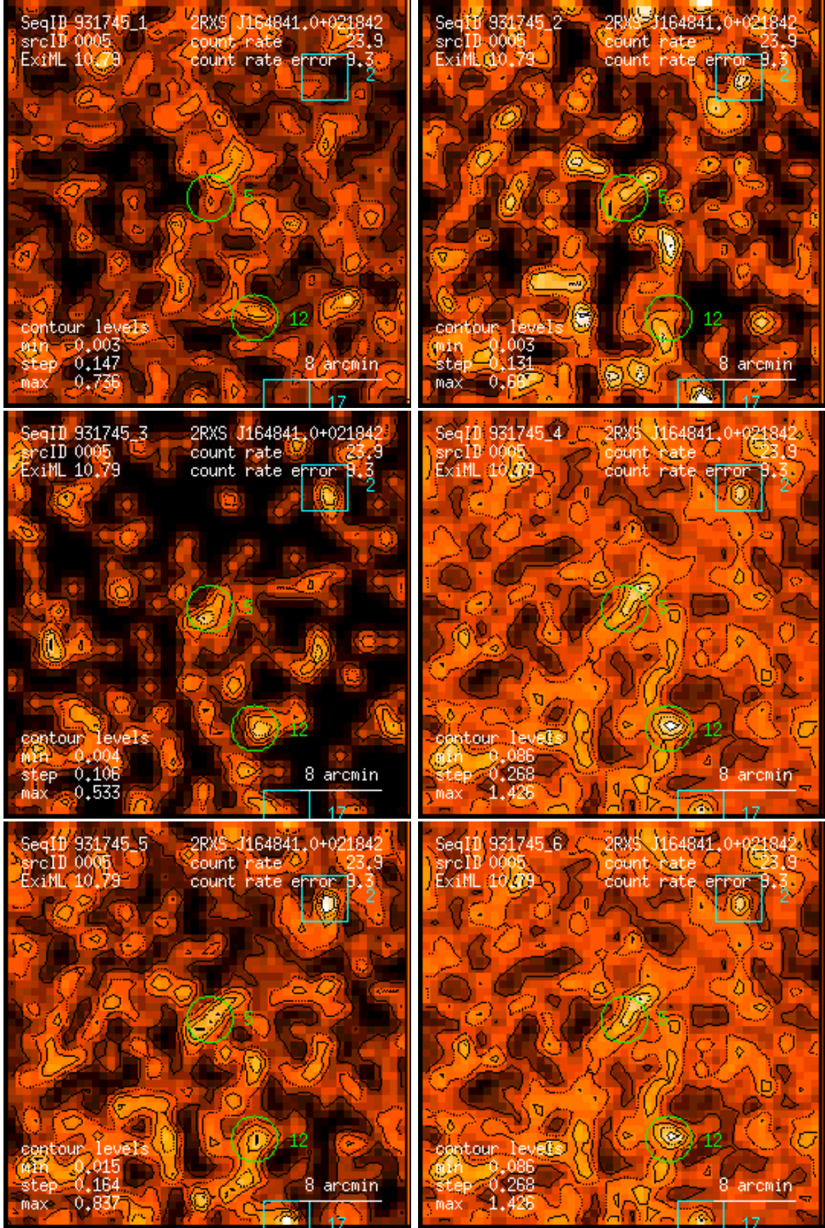
Figure 5: RASS 931745: detection 0005: band rate images, Gaussian filter: (1) PSPC channels 11 – 41, (2) 52 – 90, (3) 91 – 201, (4) 11 – 235, (5) 52 – 201, (6) 11 – 201. Broad band rates in counts/ks. Band rate contour levels in counts/ks/arcmin 2 .
