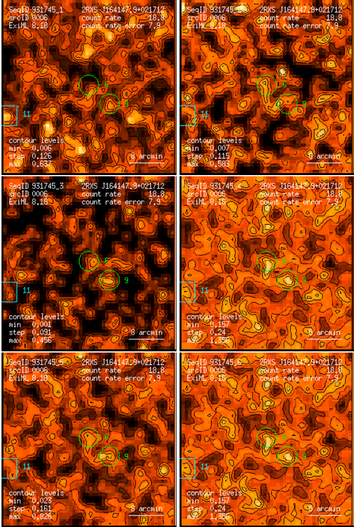
Figure 6: RASS 931745: detection 0006: band rate images, Gaussian filter: (1) PSPC channels 11 – 41, (2) 52 – 90, (3) 91 – 201, (4) 11 – 235, (5) 52 – 201, (6) 11 – 201. Broad band rates in counts/ks. Band rate contour levels in counts/ks/arcmin 2 .
