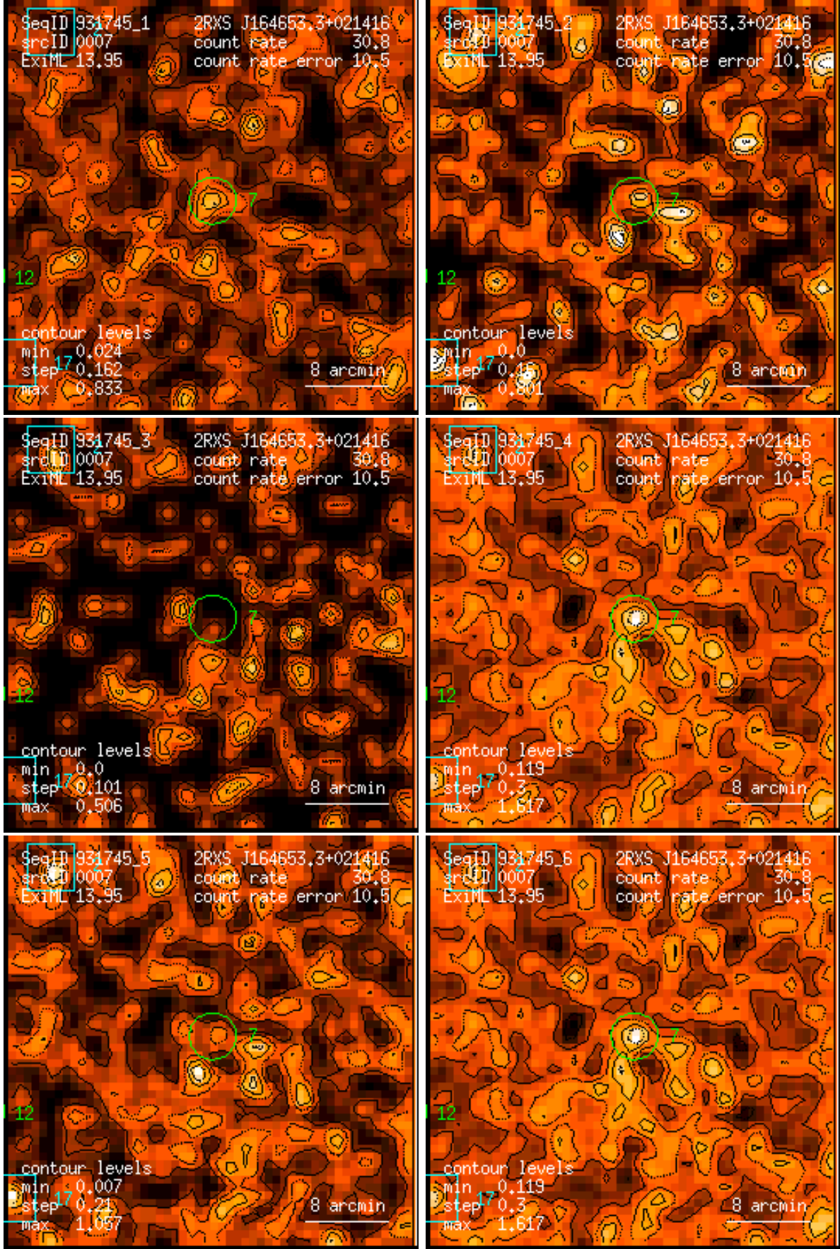
Figure 7: RASS 931745: detection 0007: band rate images, Gaussian filter: (1) PSPC channels 11 – 41, (2) 52 – 90, (3) 91 – 201, (4) 11 – 235, (5) 52 – 201, (6) 11 – 201. Broad band rates in counts/ks. Band rate contour levels in counts/ks/arcmin 2 .
