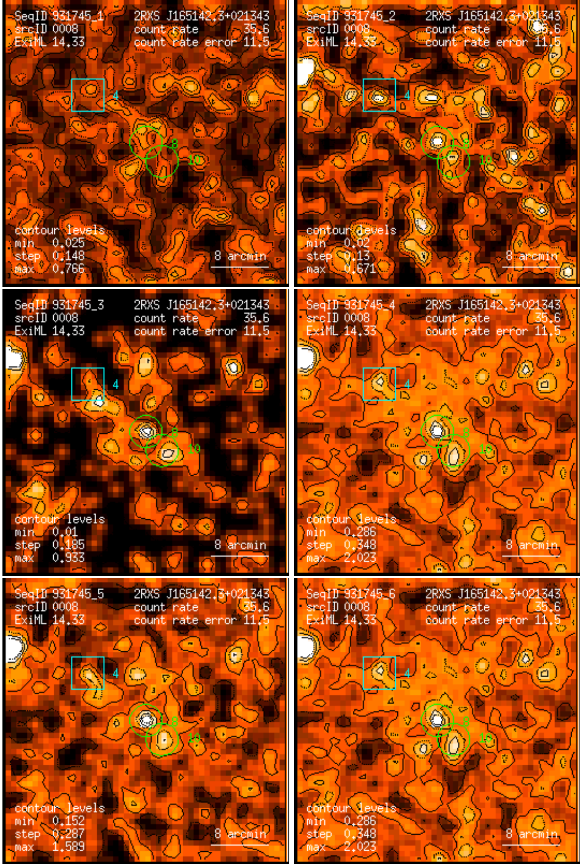
Figure 8: RASS 931745: detection 0008: band rate images, Gaussian filter: (1) PSPC channels 11 – 41, (2) 52 – 90, (3) 91 – 201, (4) 11 – 235, (5) 52 – 201, (6) 11 – 201. Broad band rates in counts/ks. Band rate contour levels in counts/ks/arcmin 2 .
