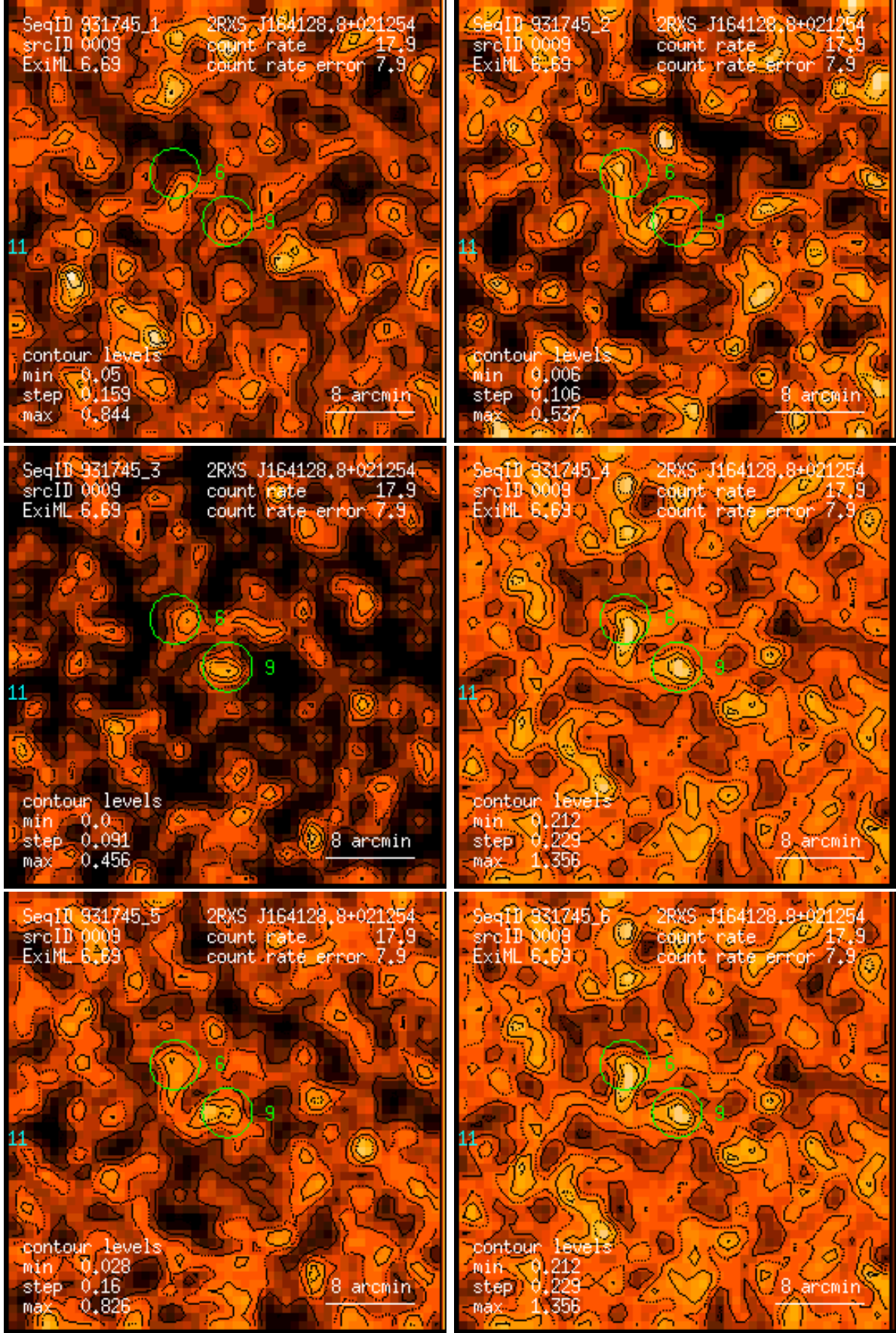
Figure 9: RASS 931745: detection 0009: band rate images, Gaussian filter: (1) PSPC channels 11 – 41, (2) 52 – 90, (3) 91 – 201, (4) 11 – 235, (5) 52 – 201, (6) 11 – 201. Broad band rates in counts/ks. Band rate contour levels in counts/ks/arcmin 2 .
