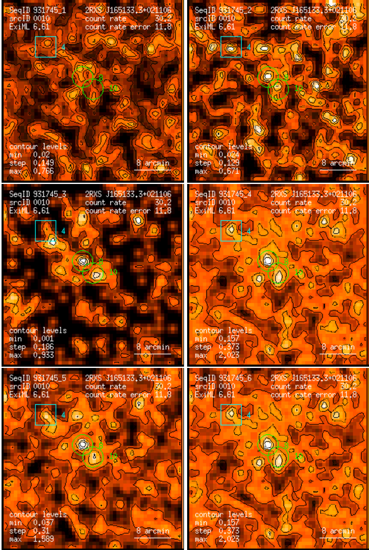
Figure 10: RASS 931745: detection 0010: band rate images, Gaussian filter: (1) PSPC channels 11 – 41, (2) 52 – 90, (3) 91 – 201, (4) 11 – 235, (5) 52 – 201, (6) 11 – 201. Broad band rates in counts/ks. Band rate contour levels in counts/ks/arcmin 2 .
