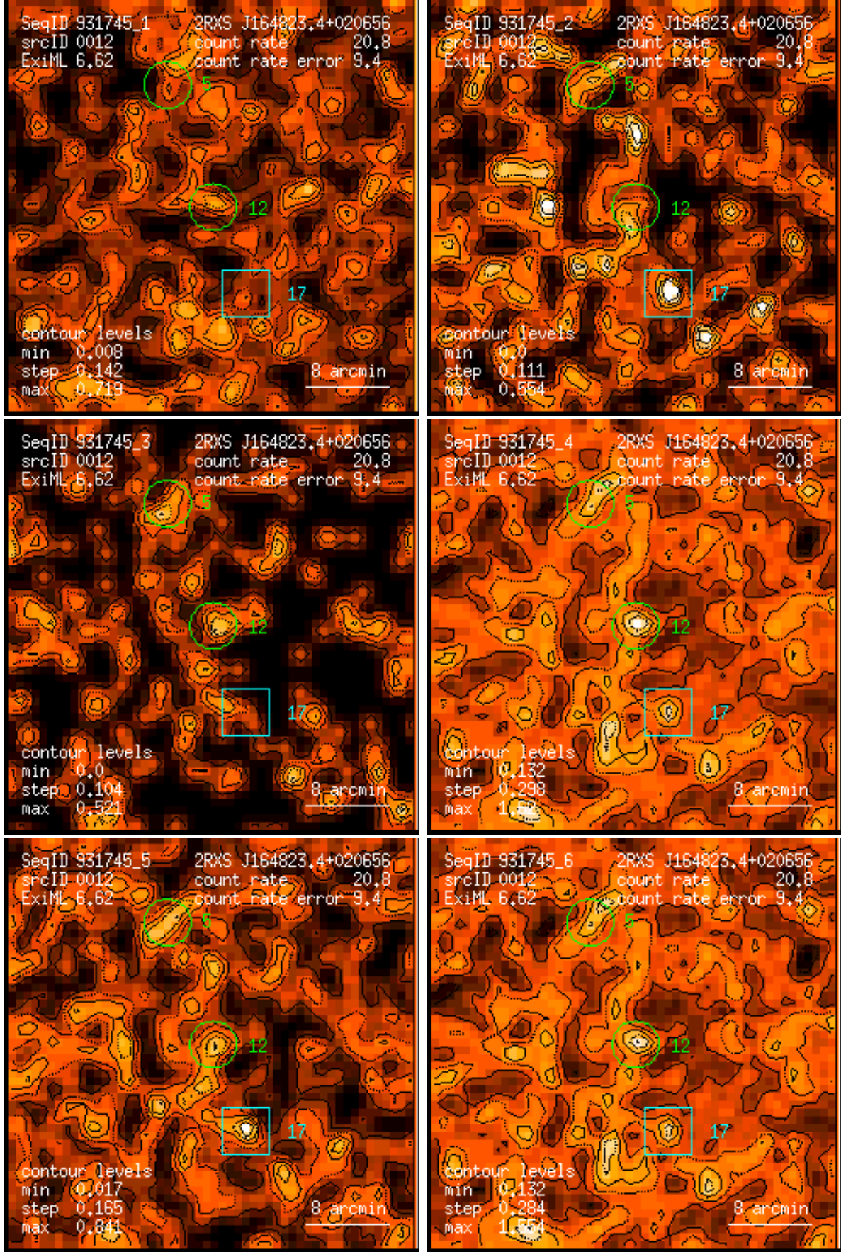
Figure 12: RASS 931745: detection 0012: band rate images, Gaussian filter: (1) PSPC channels 11 – 41, (2) 52 – 90, (3) 91 – 201, (4) 11 – 235, (5) 52 – 201, (6) 11 – 201. Broad band rates in counts/ks. Band rate contour levels in counts/ks/arcmin 2 .
