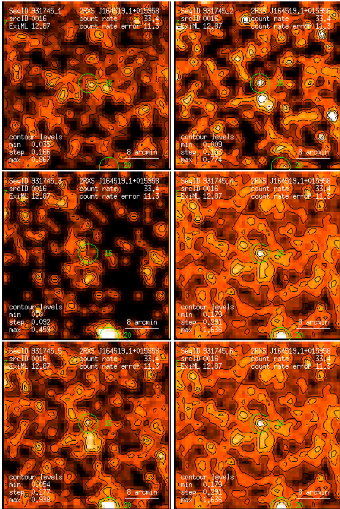
Figure 16: RASS 931745: detection 0016: band rate images, Gaussian filter: (1) PSPC channels 11 – 41, (2) 52 – 90, (3) 91 – 201, (4) 11 – 235, (5) 52 – 201, (6) 11 – 201. Broad band rates in counts/ks. Band rate contour levels in counts/ks/arcmin 2 .
