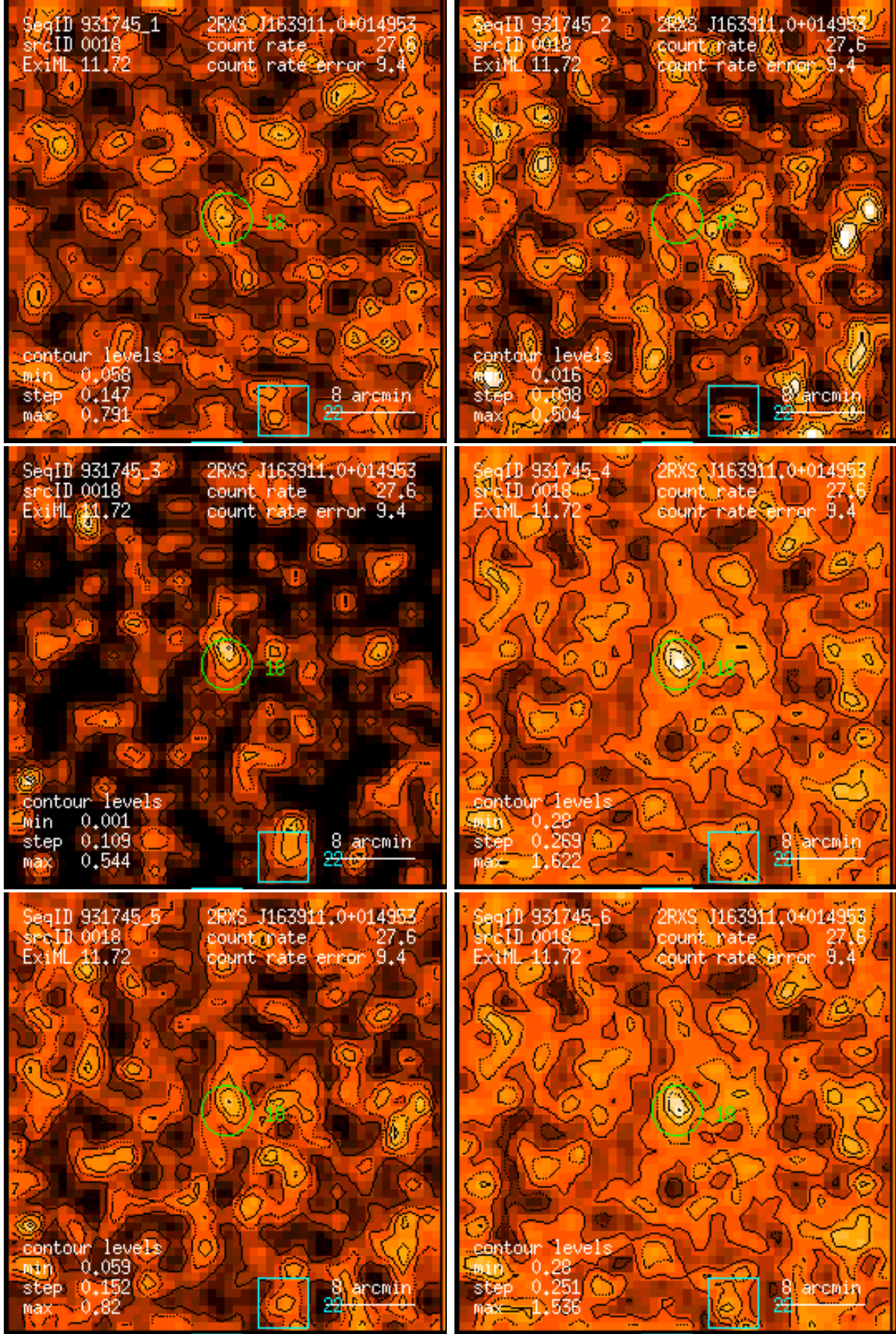
Figure 18: RASS 931745: detection 0018: band rate images, Gaussian filter: (1) PSPC channels 11 – 41, (2) 52 – 90, (3) 91 – 201, (4) 11 – 235, (5) 52 – 201, (6) 11 – 201. Broad band rates in counts/ks. Band rate contour levels in counts/ks/arcmin 2 .
