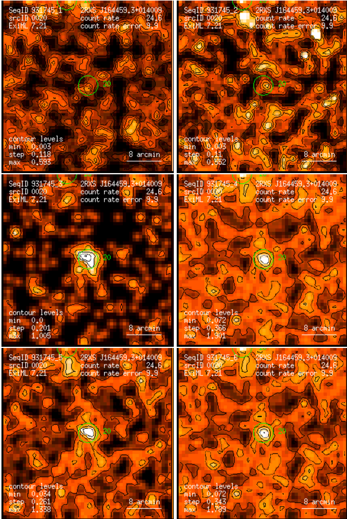
Figure 20: RASS 931745: detection 0020: band rate images, Gaussian filter: (1) PSPC channels 11 – 41, (2) 52 – 90, (3) 91 – 201, (4) 11 – 235, (5) 52 – 201, (6) 11 – 201. Broad band rates in counts/ks. Band rate contour levels in counts/ks/arcmin 2 .
