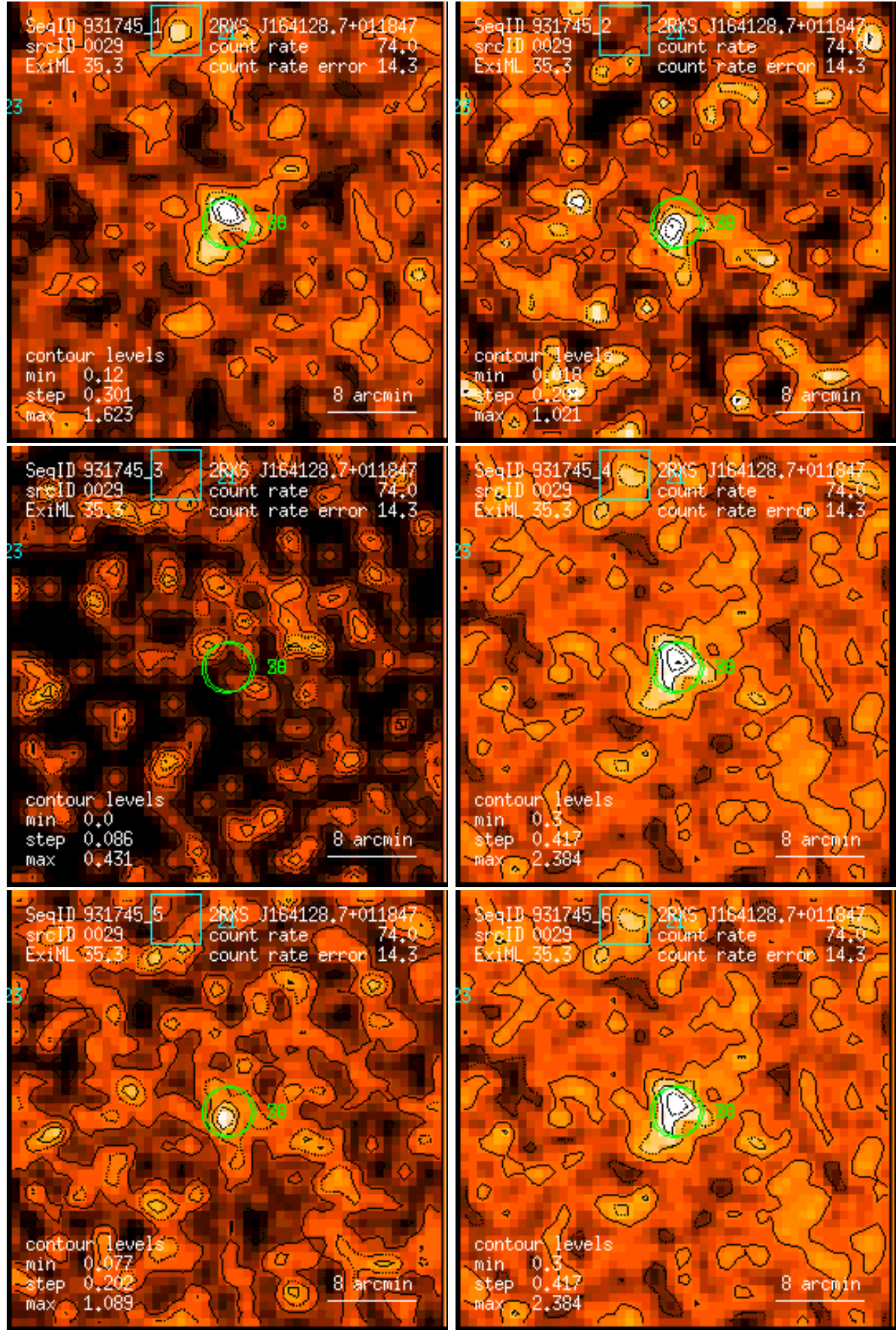
Figure 29: RASS 931745: detection 0029: band rate images, Gaussian filter: (1) PSPC channels 11 – 41, (2) 52 – 90, (3) 91 – 201, (4) 11 – 235, (5) 52 – 201, (6) 11 – 201. Broad band rates in counts/ks. Band rate contour levels in counts/ks/arcmin 2 .
