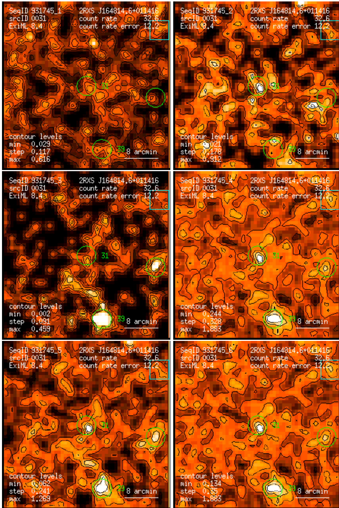
Figure 31: RASS 931745: detection 0031: band rate images, Gaussian filter: (1) PSPC channels 11 – 41, (2) 52 – 90, (3) 91 – 201, (4) 11 – 235, (5) 52 – 201, (6) 11 – 201. Broad band rates in counts/ks. Band rate contour levels in counts/ks/arcmin 2 .
