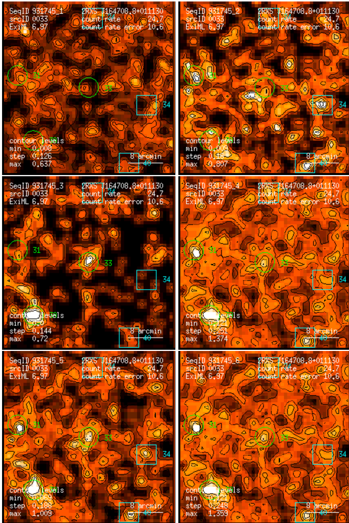
Figure 33: RASS 931745: detection 0033: band rate images, Gaussian filter: (1) PSPC channels 11 – 41, (2) 52 – 90, (3) 91 – 201, (4) 11 – 235, (5) 52 – 201, (6) 11 – 201. Broad band rates in counts/ks. Band rate contour levels in counts/ks/arcmin 2 .
