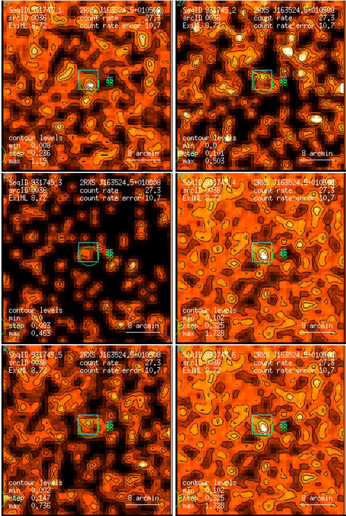
Figure 36: RASS 931745: detection 0036: band rate images, Gaussian filter: (1) PSPC channels 11 – 41, (2) 52 – 90, (3) 91 – 201, (4) 11 – 235, (5) 52 – 201, (6) 11 – 201. Broad band rates in counts/ks. Band rate contour levels in counts/ks/arcmin 2 .
