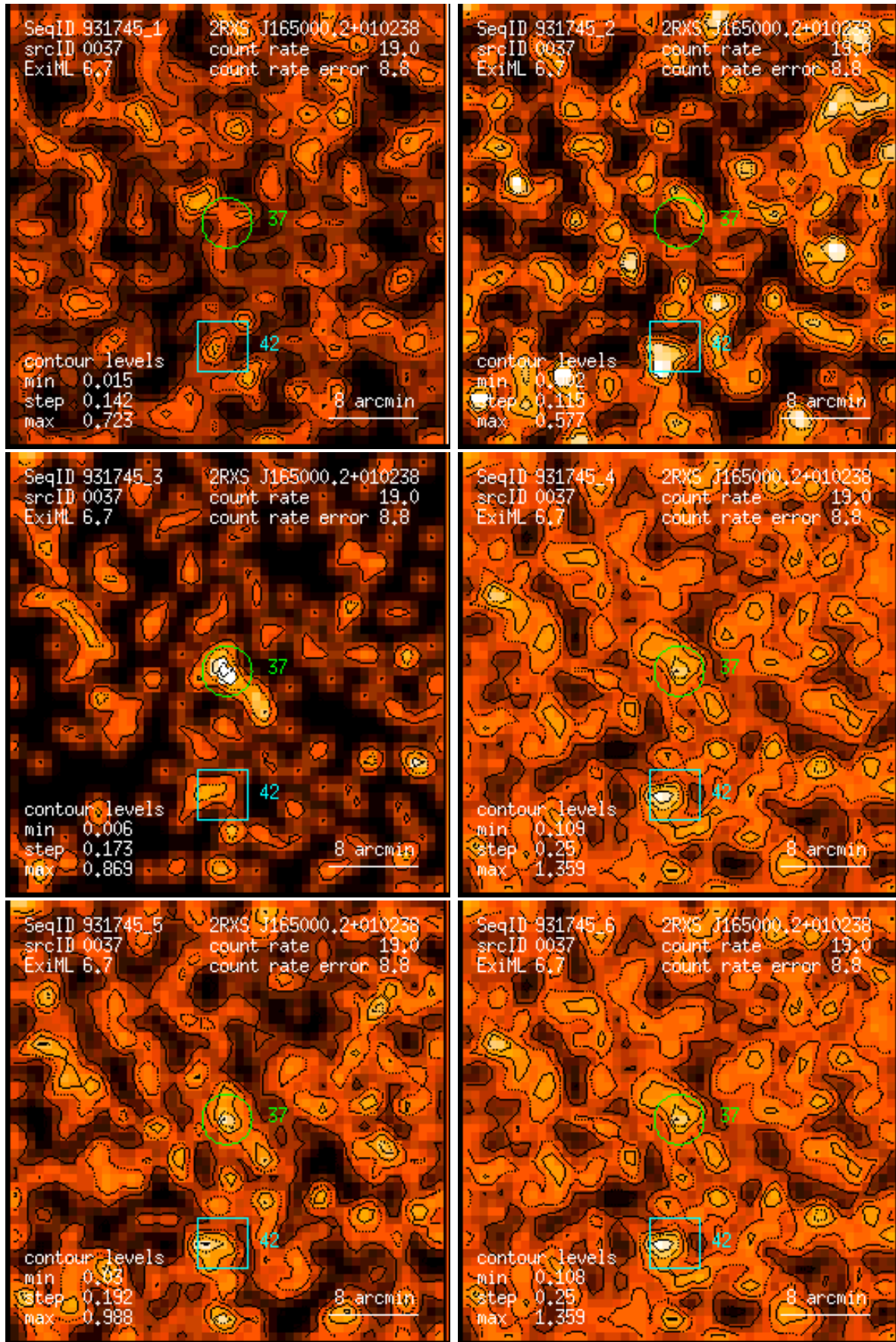
Figure 37: RASS 931745: detection 0037: band rate images, Gaussian filter: (1) PSPC channels 11 – 41, (2) 52 – 90, (3) 91 – 201, (4) 11 – 235, (5) 52 – 201, (6) 11 – 201. Broad band rates in counts/ks. Band rate contour levels in counts/ks/arcmin 2 .
