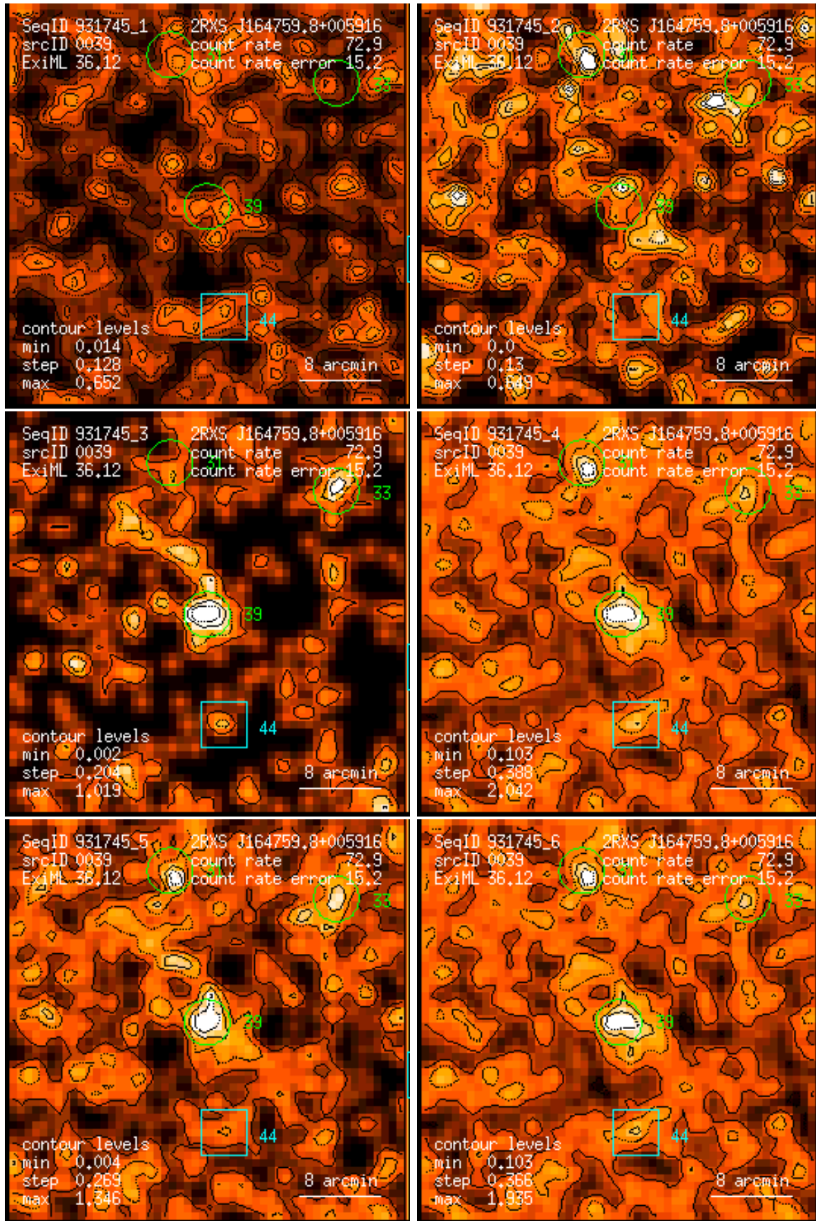
Figure 39: RASS 931745: detection 0039: band rate images, Gaussian filter: (1) PSPC channels 11 – 41, (2) 52 – 90, (3) 91 – 201, (4) 11 – 235, (5) 52 – 201, (6) 11 – 201. Broad band rates in counts/ks. Band rate contour levels in counts/ks/arcmin 2 .
