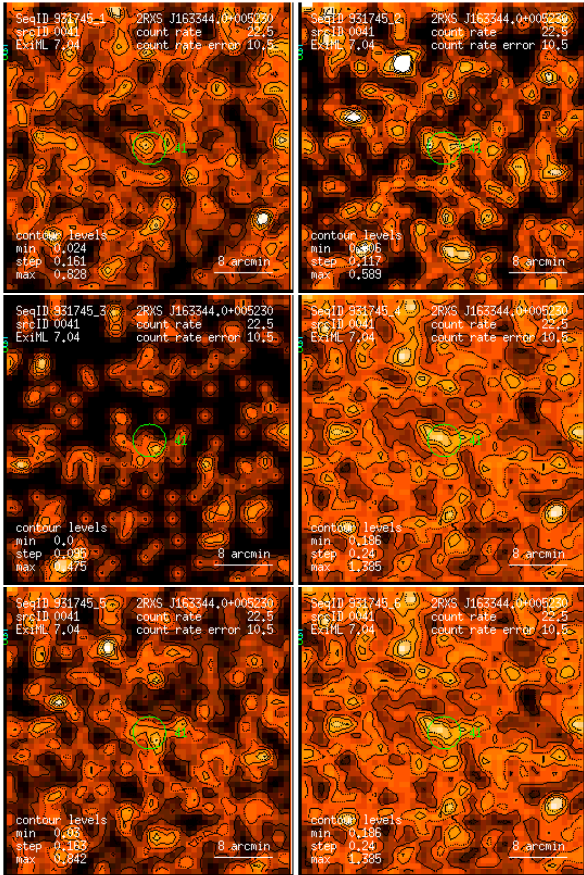
Figure 41: RASS 931745: detection 0041: band rate images, Gaussian filter: (1) PSPC channels 11 – 41, (2) 52 – 90, (3) 91 – 201, (4) 11 – 235, (5) 52 – 201, (6) 11 – 201. Broad band rates in counts/ks. Band rate contour levels in counts/ks/arcmin 2 .
