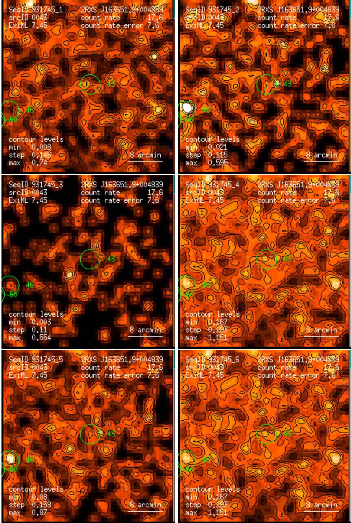
Figure 43: RASS 931745: detection 0043: band rate images, Gaussian filter: (1) PSPC channels 11 – 41, (2) 52 – 90, (3) 91 – 201, (4) 11 – 235, (5) 52 – 201, (6) 11 – 201. Broad band rates in counts/ks. Band rate contour levels in counts/ks/arcmin 2 .
