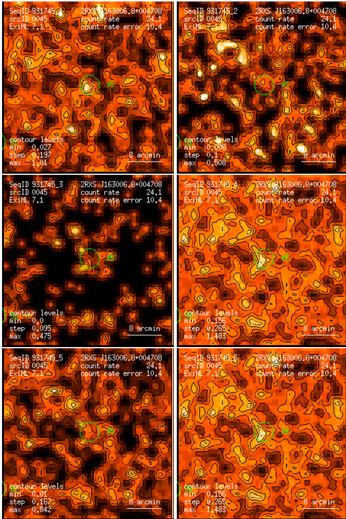
Figure 45: RASS 931745: detection 0045: band rate images, Gaussian filter: (1) PSPC channels 11 – 41, (2) 52 – 90, (3) 91 – 201, (4) 11 – 235, (5) 52 – 201, (6) 11 – 201. Broad band rates in counts/ks. Band rate contour levels in counts/ks/arcmin 2 .
