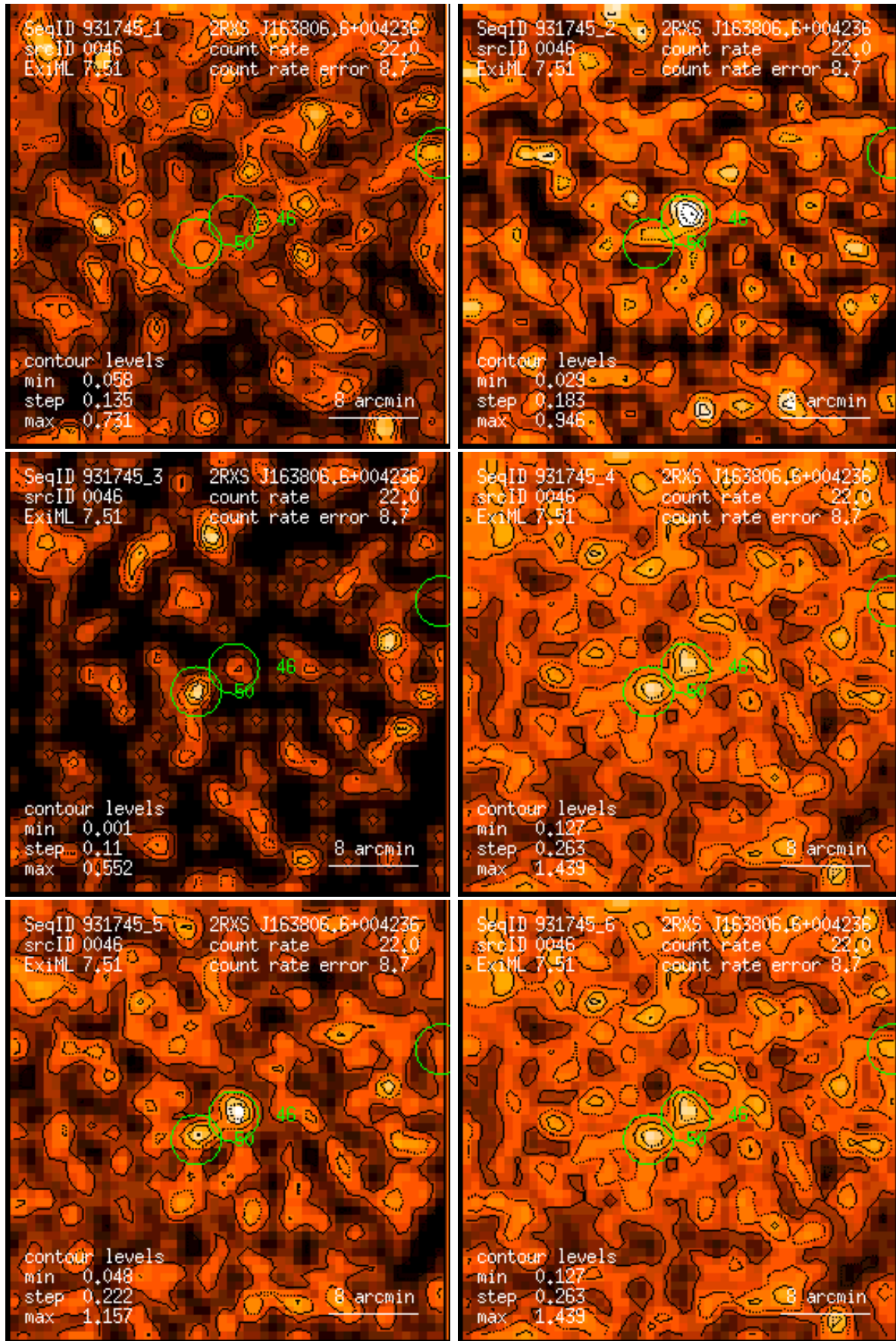
Figure 46: RASS 931745: detection 0046: band rate images, Gaussian filter: (1) PSPC channels 11 – 41, (2) 52 – 90, (3) 91 – 201, (4) 11 – 235, (5) 52 – 201, (6) 11 – 201. Broad band rates in counts/ks. Band rate contour levels in counts/ks/arcmin 2 .
