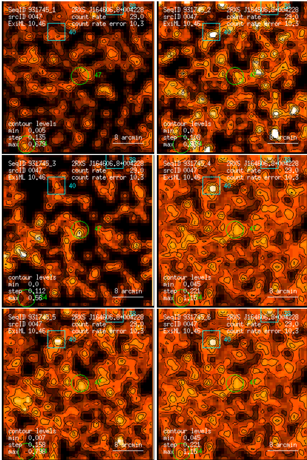
Figure 47: RASS 931745: detection 0047: band rate images, Gaussian filter: (1) PSPC channels 11 – 41, (2) 52 – 90, (3) 91 – 201, (4) 11 – 235, (5) 52 – 201, (6) 11 – 201. Broad band rates in counts/ks. Band rate contour levels in counts/ks/arcmin 2 .
