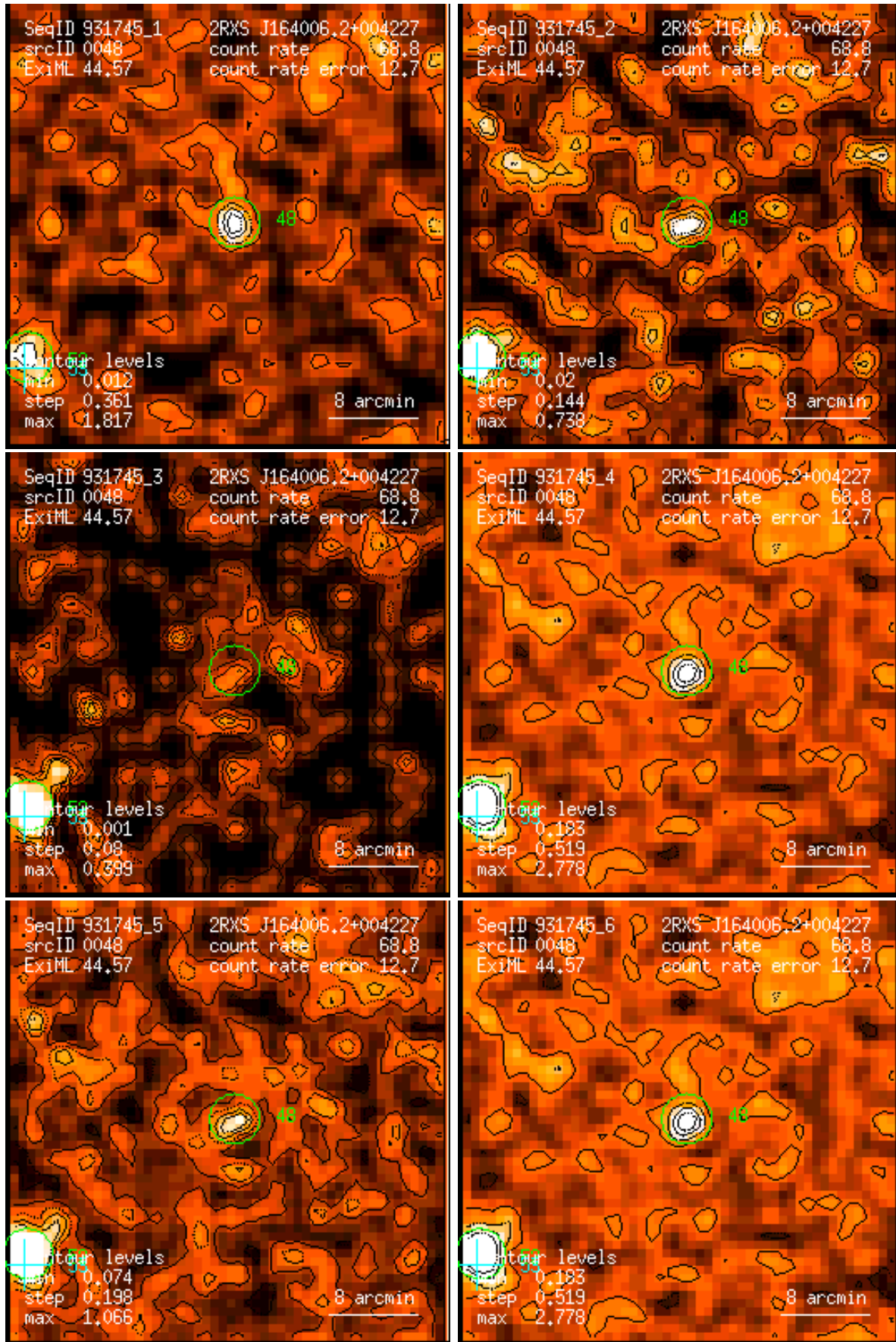
Figure 48: RASS 931745: detection 0048: band rate images, Gaussian filter: (1) PSPC channels 11 – 41, (2) 52 – 90, (3) 91 – 201, (4) 11 – 235, (5) 52 – 201, (6) 11 – 201. Broad band rates in counts/ks. Band rate contour levels in counts/ks/arcmin 2 .
