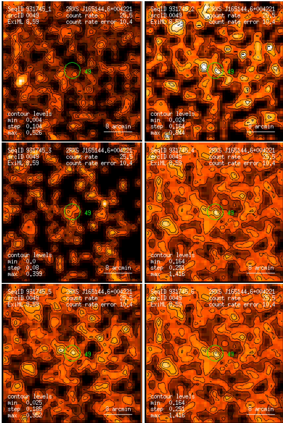
Figure 49: RASS 931745: detection 0049: band rate images, Gaussian filter: (1) PSPC channels 11 – 41, (2) 52 – 90, (3) 91 – 201, (4) 11 – 235, (5) 52 – 201, (6) 11 – 201. Broad band rates in counts/ks. Band rate contour levels in counts/ks/arcmin 2 .
