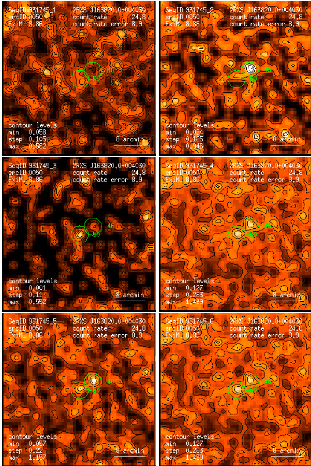
Figure 50: RASS 931745: detection 0050: band rate images, Gaussian filter: (1) PSPC channels 11 – 41, (2) 52 – 90, (3) 91 – 201, (4) 11 – 235, (5) 52 – 201, (6) 11 – 201. Broad band rates in counts/ks. Band rate contour levels in counts/ks/arcmin 2 .
