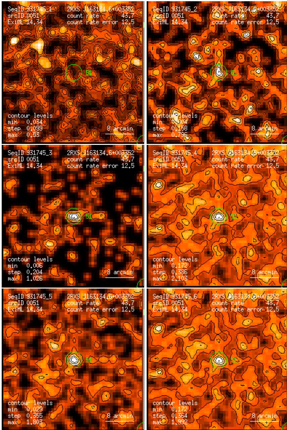
Figure 51: RASS 931745: detection 0051: band rate images, Gaussian filter: (1) PSPC channels 11 – 41, (2) 52 – 90, (3) 91 – 201, (4) 11 – 235, (5) 52 – 201, (6) 11 – 201. Broad band rates in counts/ks. Band rate contour levels in counts/ks/arcmin 2 .
