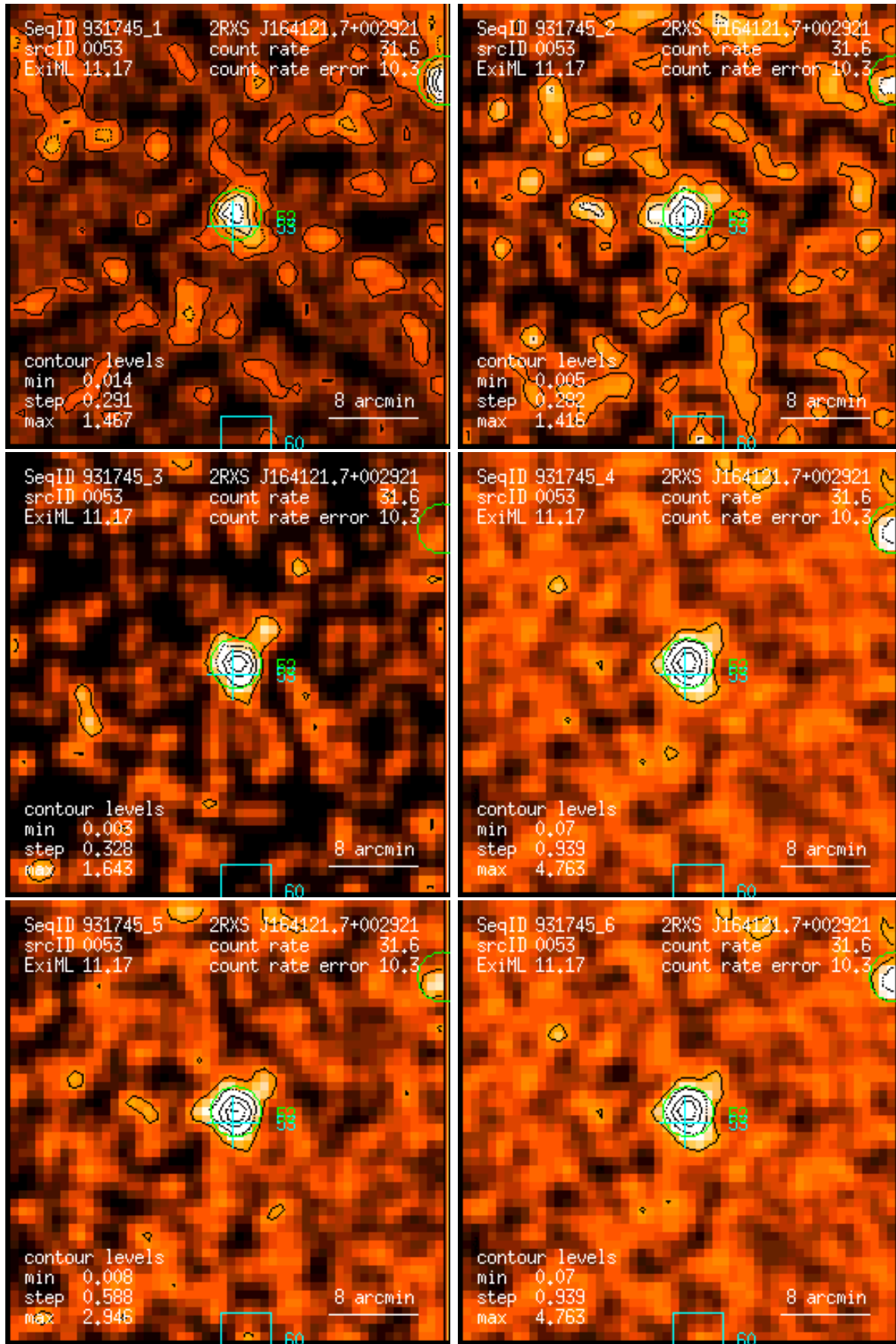
Figure 53: RASS 931745: detection 0053: band rate images, Gaussian filter: (1) PSPC channels 11 – 41, (2) 52 – 90, (3) 91 – 201, (4) 11 – 235, (5) 52 – 201, (6) 11 – 201. Broad band rates in counts/ks. Band rate contour levels in counts/ks/arcmin 2 .
