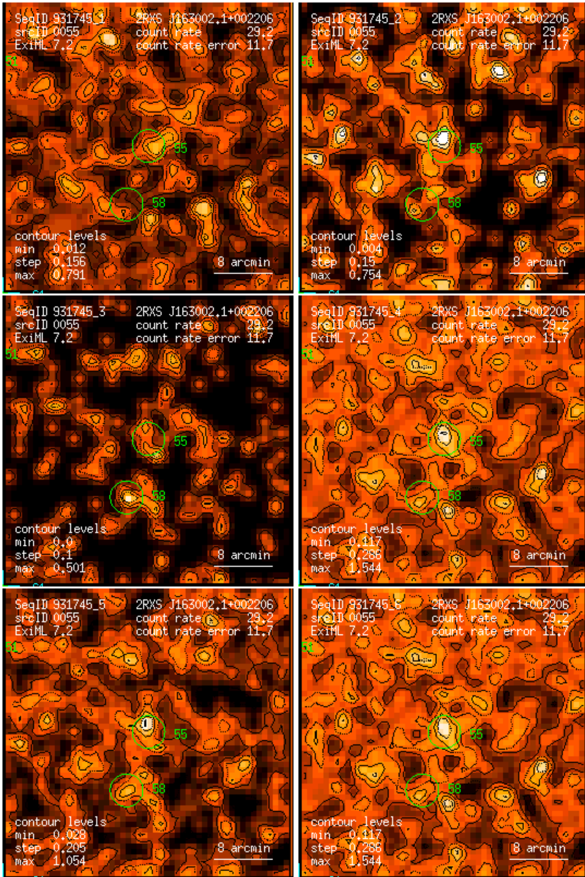
Figure 55: RASS 931745: detection 0055: band rate images, Gaussian filter: (1) PSPC channels 11 – 41, (2) 52 – 90, (3) 91 – 201, (4) 11 – 235, (5) 52 – 201, (6) 11 – 201. Broad band rates in counts/ks. Band rate contour levels in counts/ks/arcmin 2 .
