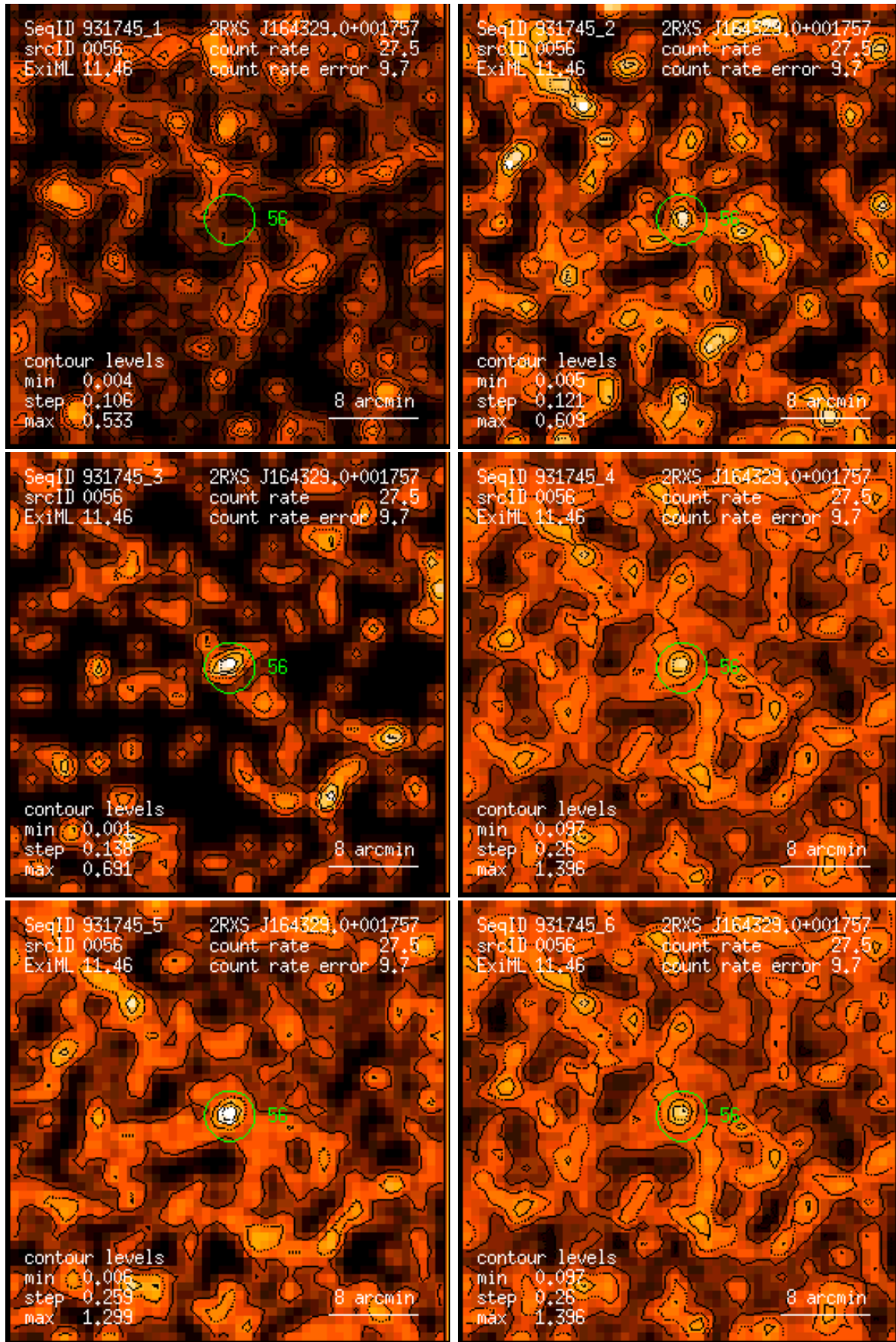
Figure 56: RASS 931745: detection 0056: band rate images, Gaussian filter: (1) PSPC channels 11 – 41, (2) 52 – 90, (3) 91 – 201, (4) 11 – 235, (5) 52 – 201, (6) 11 – 201. Broad band rates in counts/ks. Band rate contour levels in counts/ks/arcmin 2 .
