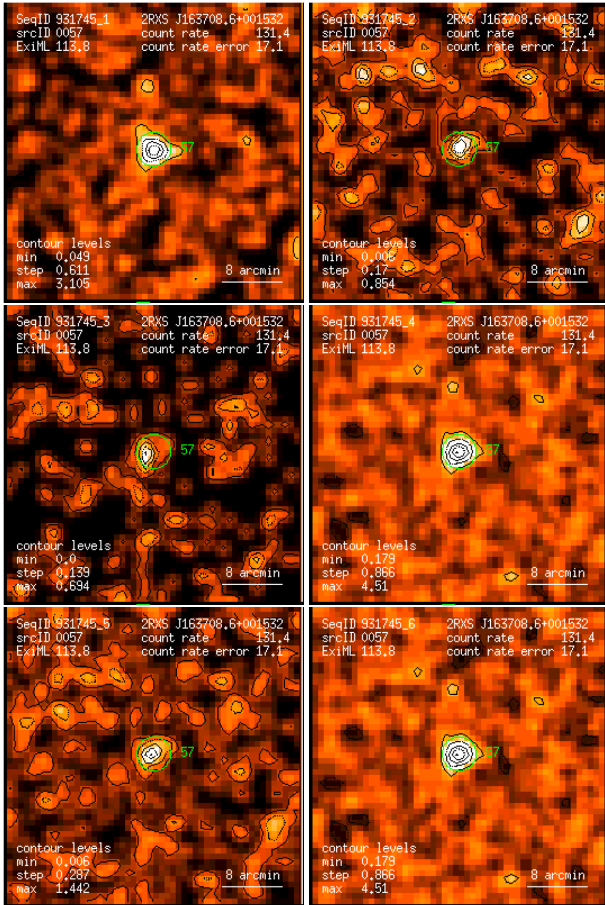
Figure 57: RASS 931745: detection 0057: band rate images, Gaussian filter: (1) PSPC channels 11 – 41, (2) 52 – 90, (3) 91 – 201, (4) 11 – 235, (5) 52 – 201, (6) 11 – 201. Broad band rates in counts/ks. Band rate contour levels in counts/ks/arcmin 2 .
