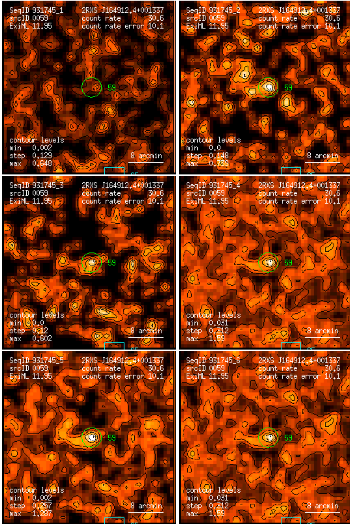
Figure 59: RASS 931745: detection 0059: band rate images, Gaussian filter: (1) PSPC channels 11 – 41, (2) 52 – 90, (3) 91 – 201, (4) 11 – 235, (5) 52 – 201, (6) 11 – 201. Broad band rates in counts/ks. Band rate contour levels in counts/ks/arcmin 2 .
