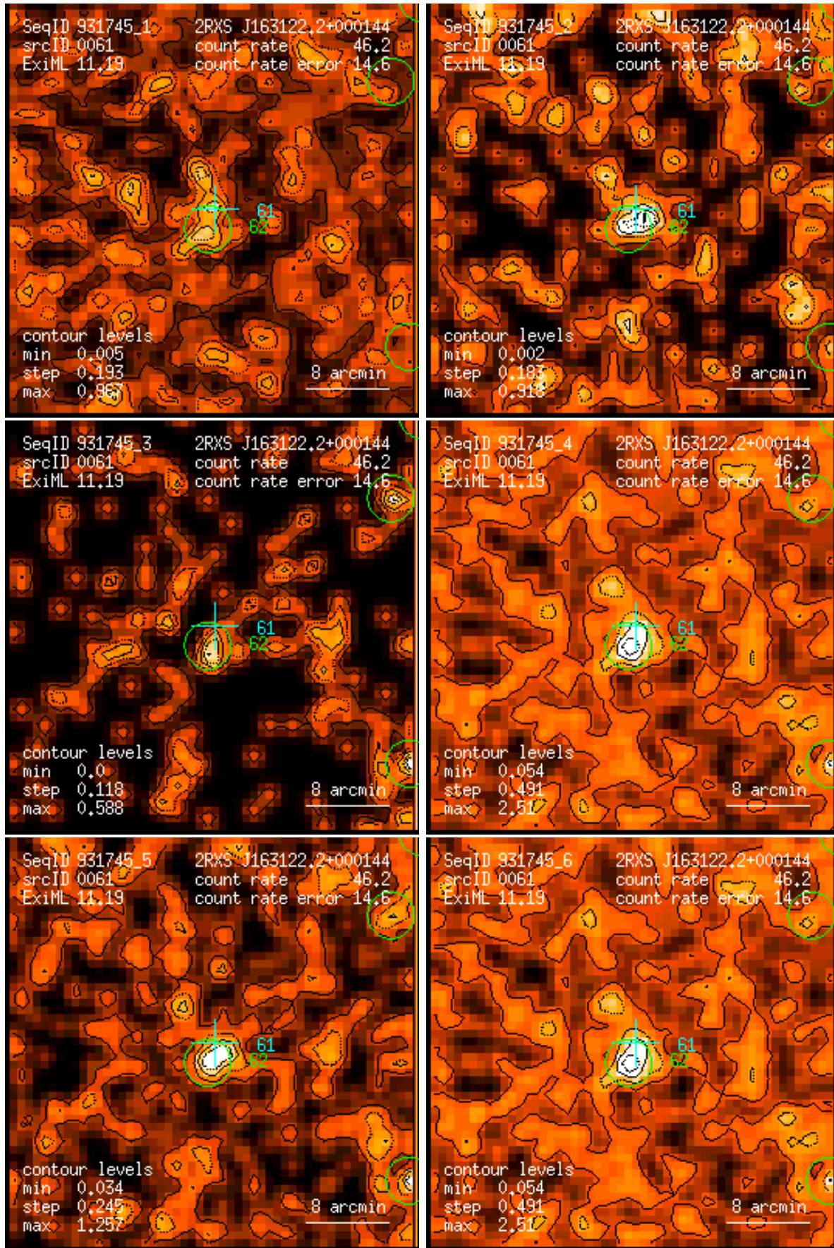
Figure 61: RASS 931745: detection 0061: band rate images, Gaussian filter: (1) PSPC channels 11 – 41, (2) 52 – 90, (3) 91 – 201, (4) 11 – 235, (5) 52 – 201, (6) 11 – 201. Broad band rates in counts/ks. Band rate contour levels in counts/ks/arcmin 2 .
