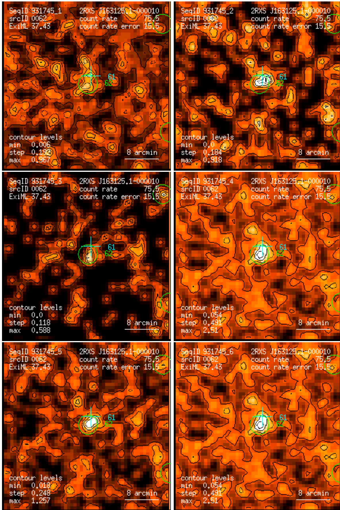
Figure 62: RASS 931745: detection 0062: band rate images, Gaussian filter: (1) PSPC channels 11 – 41, (2) 52 – 90, (3) 91 – 201, (4) 11 – 235, (5) 52 – 201, (6) 11 – 201. Broad band rates in counts/ks. Band rate contour levels in counts/ks/arcmin 2 .
