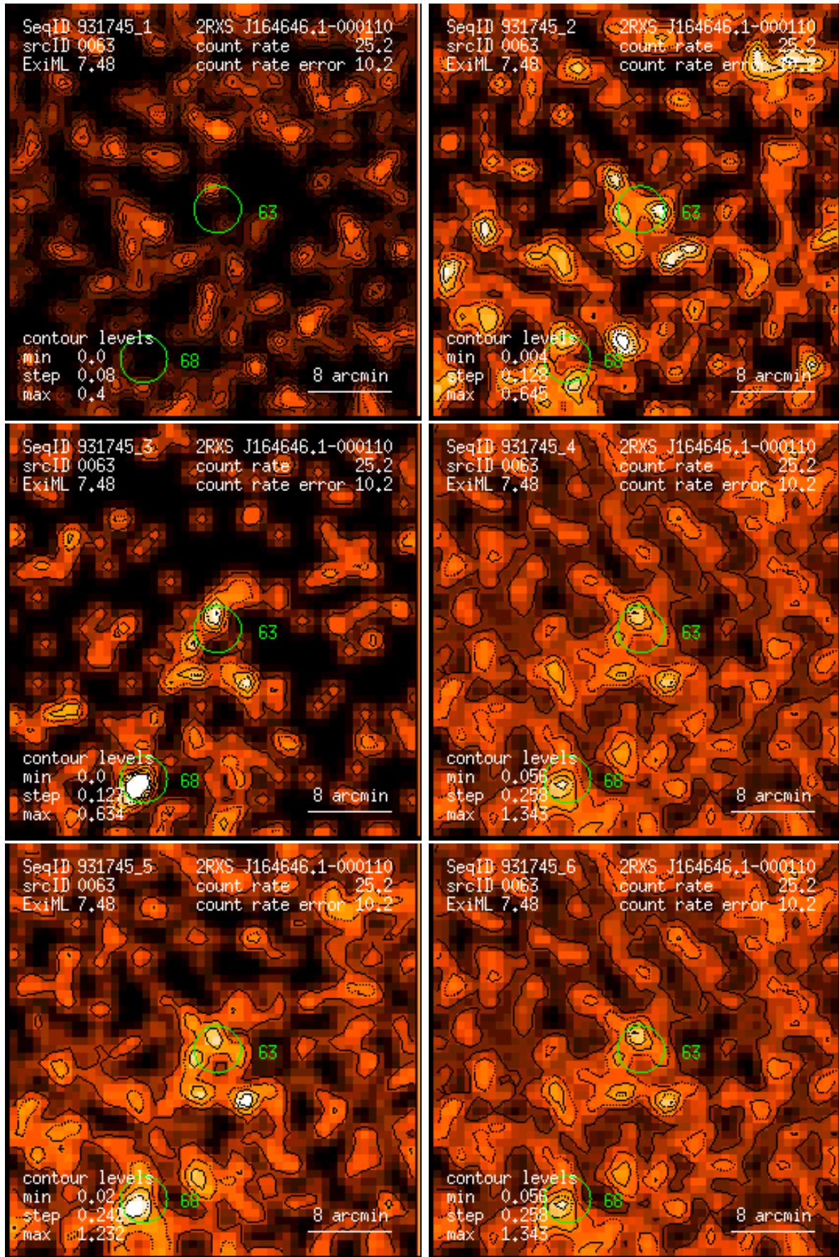
Figure 63: RASS 931745: detection 0063: band rate images, Gaussian filter: (1) PSPC channels 11 – 41, (2) 52 – 90, (3) 91 – 201, (4) 11 – 235, (5) 52 – 201, (6) 11 – 201. Broad band rates in counts/ks. Band rate contour levels in counts/ks/arcmin 2 .
