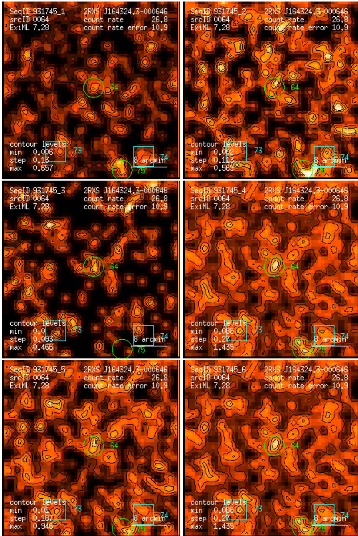
Figure 64: RASS 931745: detection 0064: band rate images, Gaussian filter: (1) PSPC channels 11 – 41, (2) 52 – 90, (3) 91 – 201, (4) 11 – 235, (5) 52 – 201, (6) 11 – 201. Broad band rates in counts/ks. Band rate contour levels in counts/ks/arcmin 2 .
