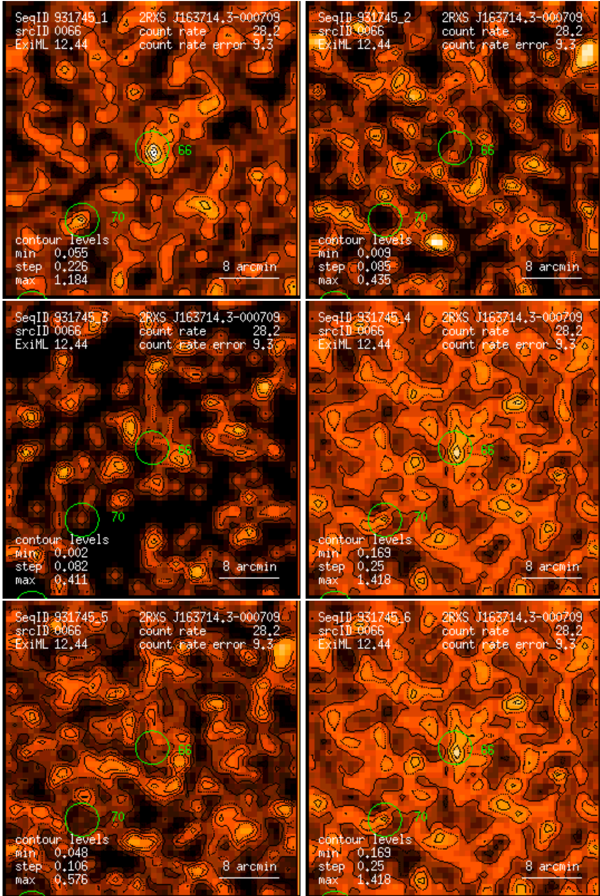
Figure 66: RASS 931745: detection 0066: band rate images, Gaussian filter: (1) PSPC channels 11 – 41, (2) 52 – 90, (3) 91 – 201, (4) 11 – 235, (5) 52 – 201, (6) 11 – 201. Broad band rates in counts/ks. Band rate contour levels in counts/ks/arcmin 2 .
