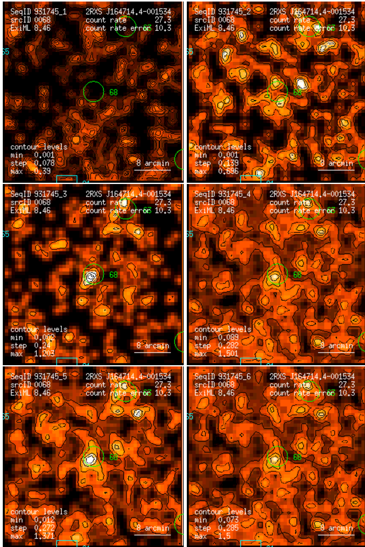
Figure 68: RASS 931745: detection 0068: band rate images, Gaussian filter: (1) PSPC channels 11 – 41, (2) 52 – 90, (3) 91 – 201, (4) 11 – 235, (5) 52 – 201, (6) 11 – 201. Broad band rates in counts/ks. Band rate contour levels in counts/ks/arcmin 2 .
