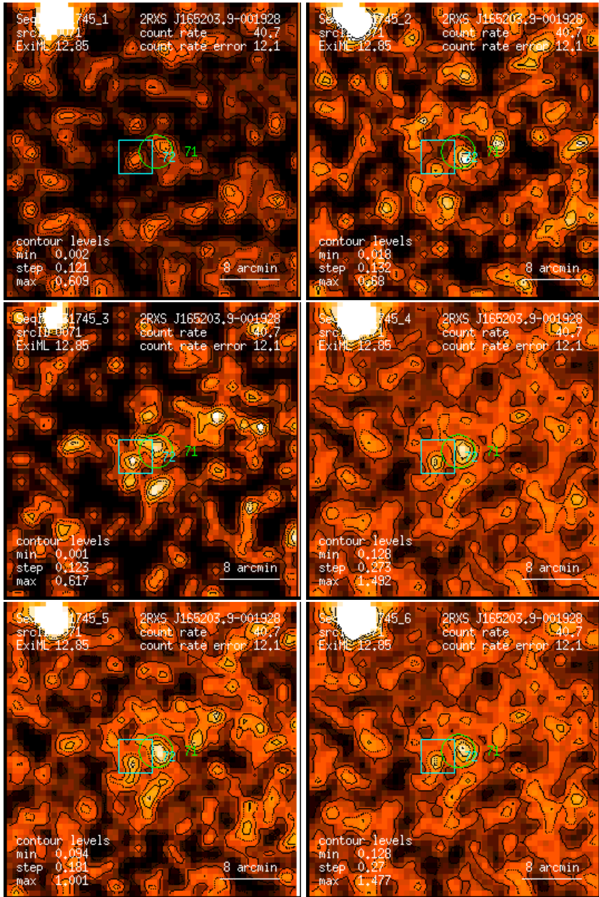
Figure 71: RASS 931745: detection 0071: band rate images, Gaussian filter: (1) PSPC channels 11 – 41, (2) 52 – 90, (3) 91 – 201, (4) 11 – 235, (5) 52 – 201, (6) 11 – 201. Broad band rates in counts/ks. Band rate contour levels in counts/ks/arcmin 2 .
