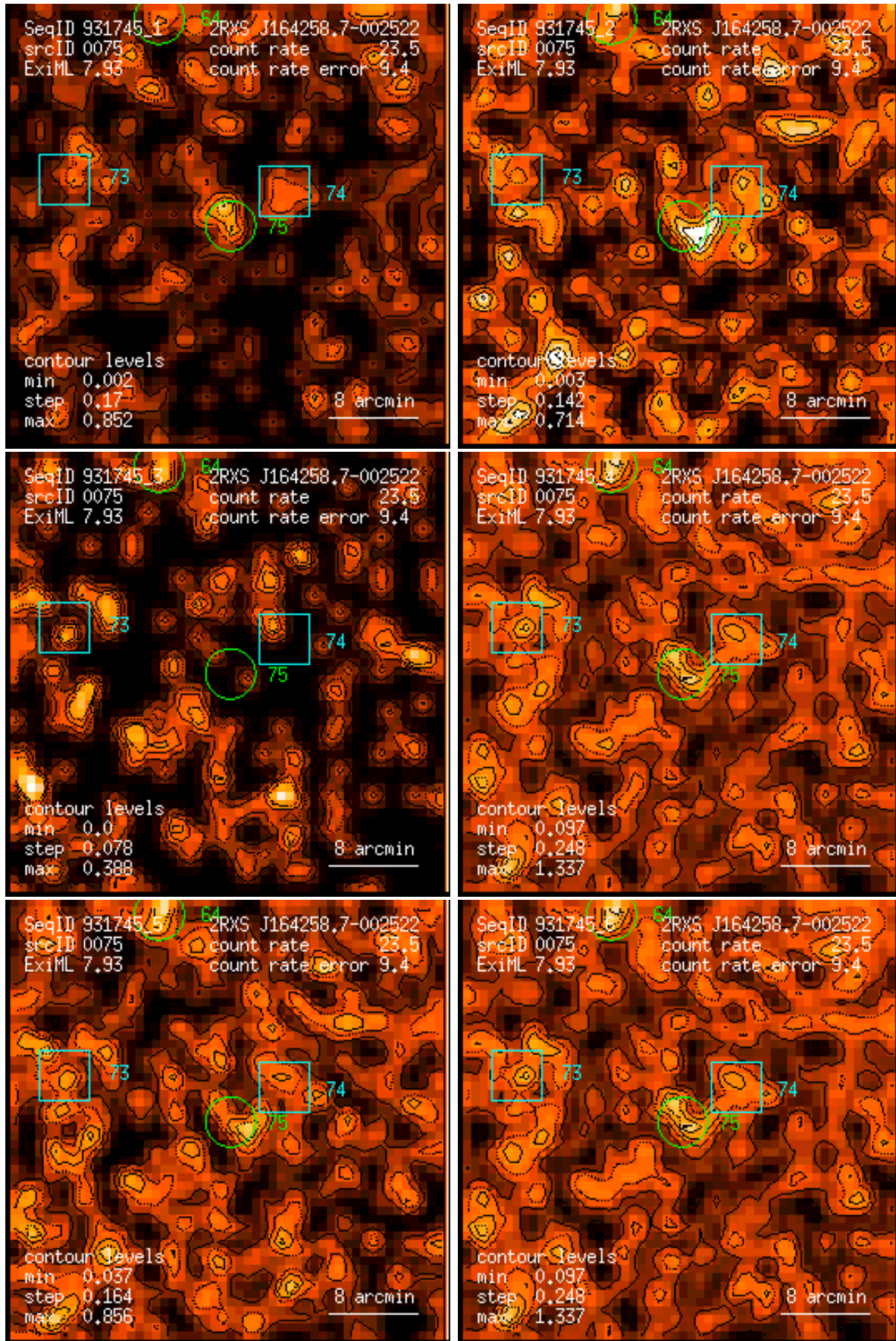
Figure 75: RASS 931745: detection 0075: band rate images, Gaussian filter: (1) PSPC channels 11 – 41, (2) 52 – 90, (3) 91 – 201, (4) 11 – 235, (5) 52 – 201, (6) 11 – 201. Broad band rates in counts/ks. Band rate contour levels in counts/ks/arcmin 2 .
