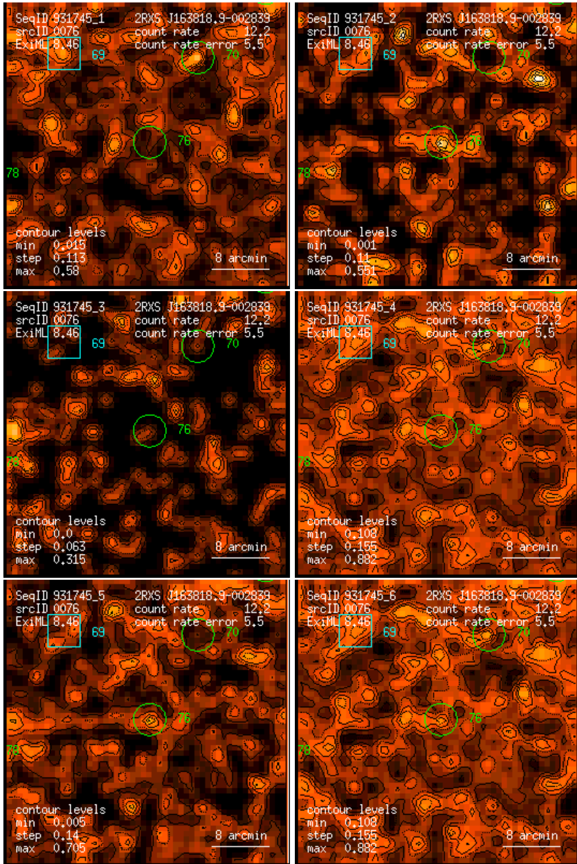
Figure 76: RASS 931745: detection 0076: band rate images, Gaussian filter: (1) PSPC channels 11 – 41, (2) 52 – 90, (3) 91 – 201, (4) 11 – 235, (5) 52 – 201, (6) 11 – 201. Broad band rates in counts/ks. Band rate contour levels in counts/ks/arcmin 2 .
