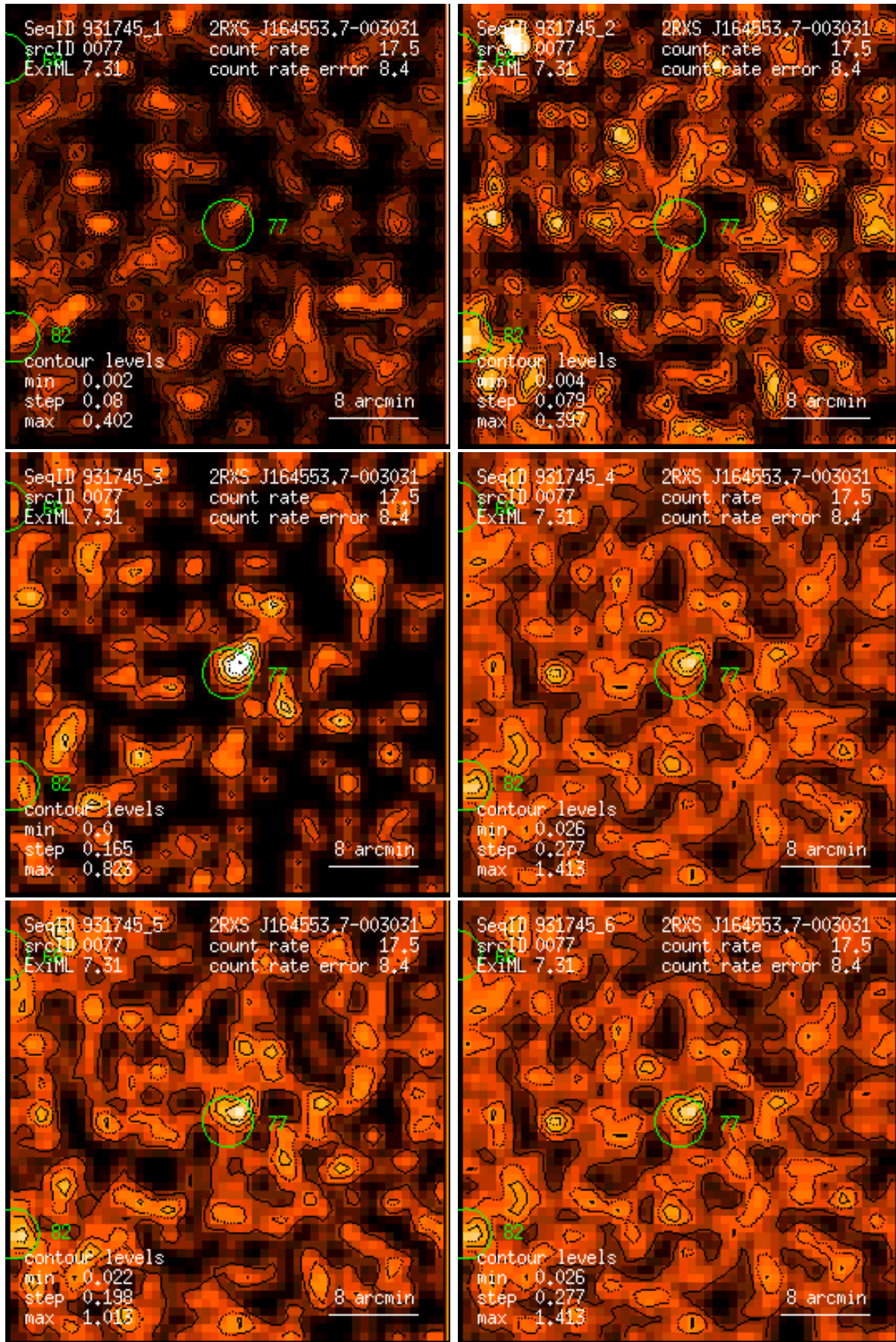
Figure 77: RASS 931745: detection 0077: band rate images, Gaussian filter: (1) PSPC channels 11 – 41, (2) 52 – 90, (3) 91 – 201, (4) 11 – 235, (5) 52 – 201, (6) 11 – 201. Broad band rates in counts/ks. Band rate contour levels in counts/ks/arcmin 2 .
