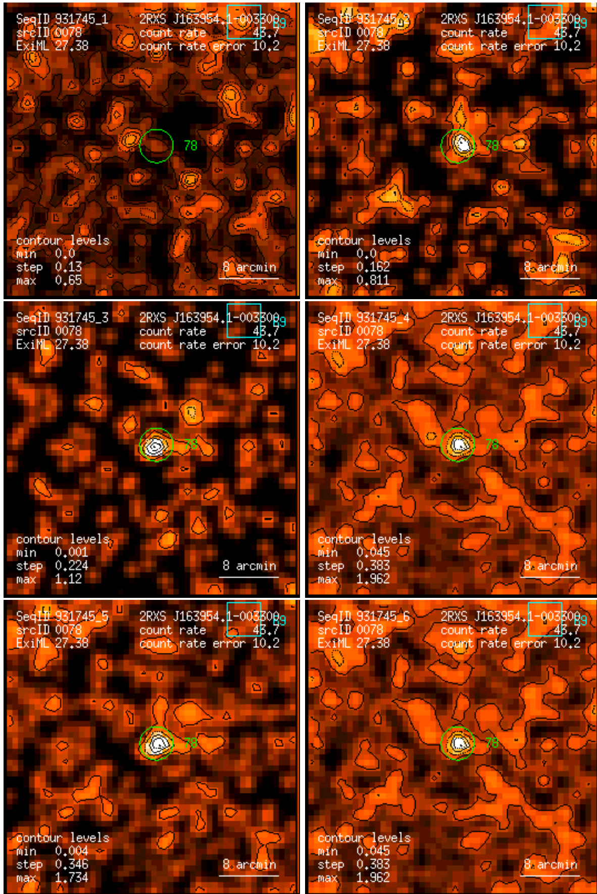
Figure 78: RASS 931745: detection 0078: band rate images, Gaussian filter: (1) PSPC channels 11 – 41, (2) 52 – 90, (3) 91 – 201, (4) 11 – 235, (5) 52 – 201, (6) 11 – 201. Broad band rates in counts/ks. Band rate contour levels in counts/ks/arcmin 2 .
