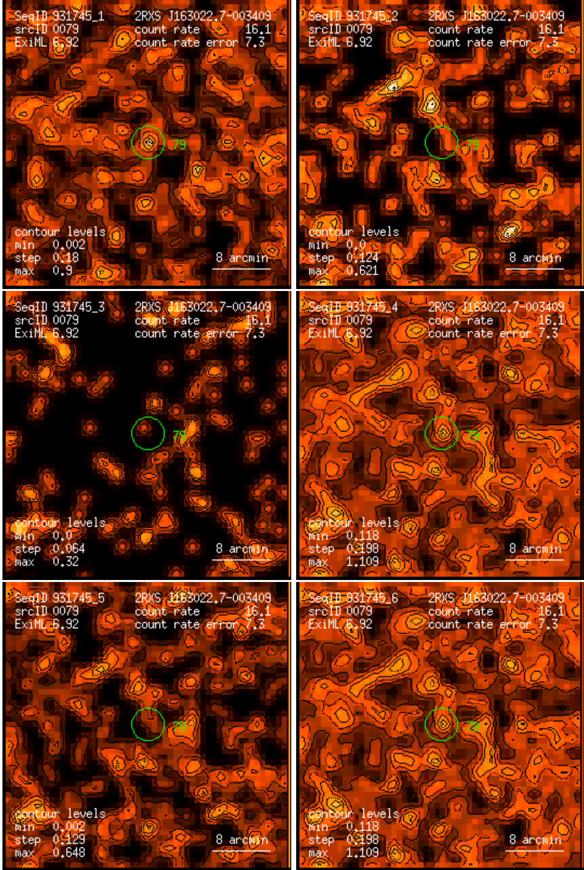
Figure 79: RASS 931745: detection 0079: band rate images, Gaussian filter: (1) PSPC channels 11 – 41, (2) 52 – 90, (3) 91 – 201, (4) 11 – 235, (5) 52 – 201, (6) 11 – 201. Broad band rates in counts/ks. Band rate contour levels in counts/ks/arcmin 2 .
