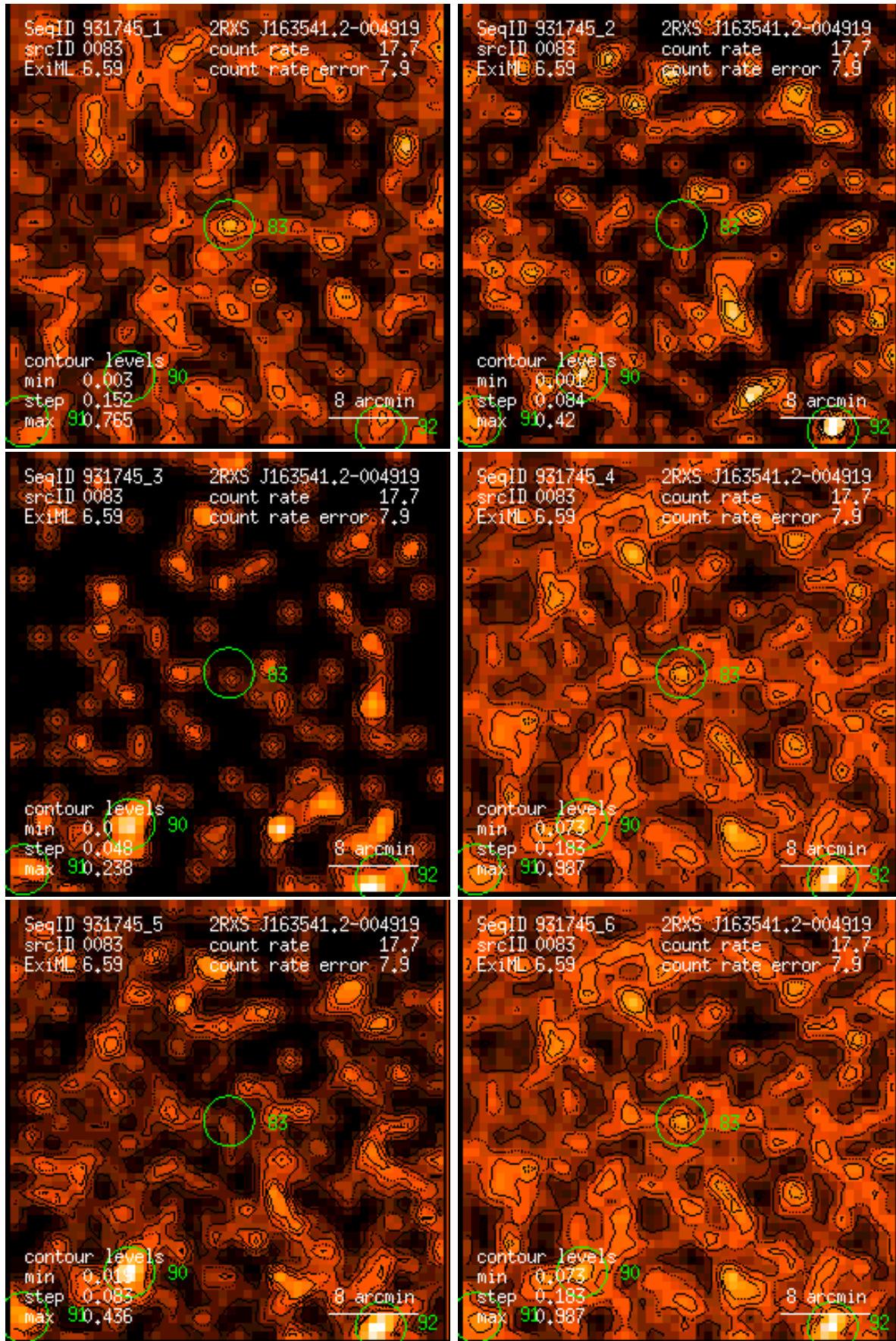
Figure 83: RASS 931745: detection 0083: band rate images, Gaussian filter: (1) PSPC channels 11 – 41, (2) 52 – 90, (3) 91 – 201, (4) 11 – 235, (5) 52 – 201, (6) 11 – 201. Broad band rates in counts/ks. Band rate contour levels in counts/ks/arcmin 2 .
