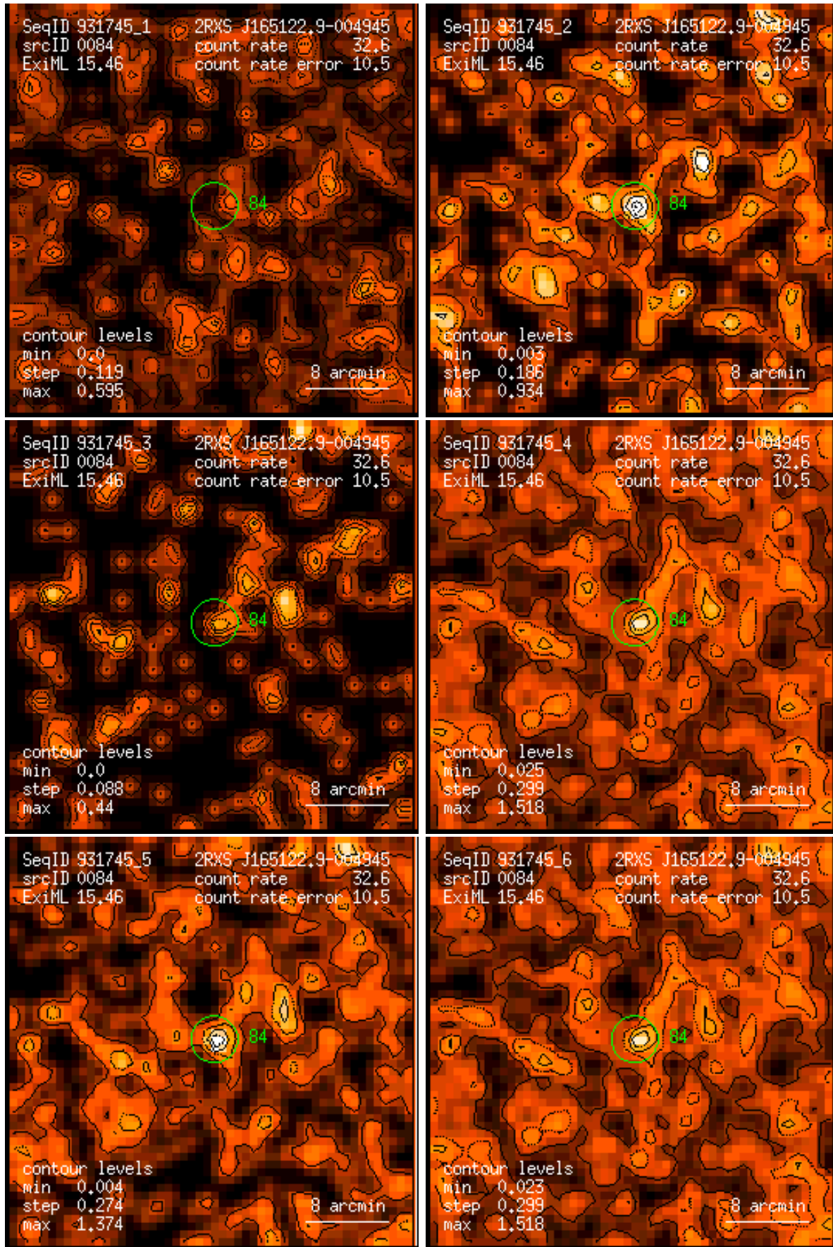
Figure 84: RASS 931745: detection 0084: band rate images, Gaussian filter: (1) PSPC channels 11 – 41, (2) 52 – 90, (3) 91 – 201, (4) 11 – 235, (5) 52 – 201, (6) 11 – 201. Broad band rates in counts/ks. Band rate contour levels in counts/ks/arcmin 2 .
