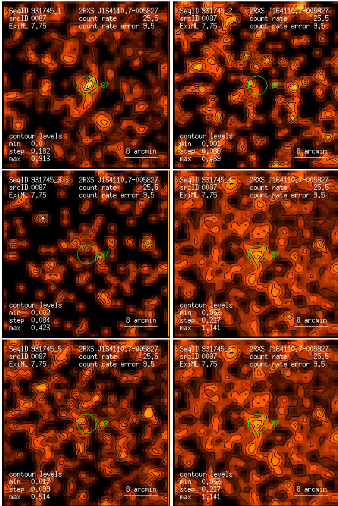
Figure 87: RASS 931745: detection 0087: band rate images, Gaussian filter: (1) PSPC channels 11 – 41, (2) 52 – 90, (3) 91 – 201, (4) 11 – 235, (5) 52 – 201, (6) 11 – 201. Broad band rates in counts/ks. Band rate contour levels in counts/ks/arcmin 2 .
